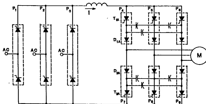
ASCII Current Source Inverter
