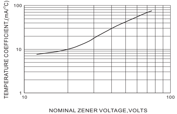
Fig. 2 TEMPERATURE COEFFICIENTS
