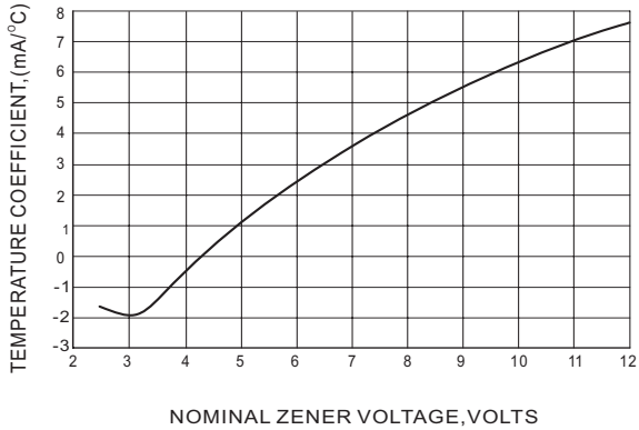
Fig. 1 TEMPERATURE COEFFICIENTS
