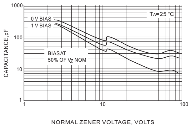
Fig. 6 TYPICAL CAPACITANCE
