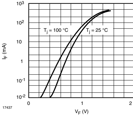
Figure 1. Forward characteristics
