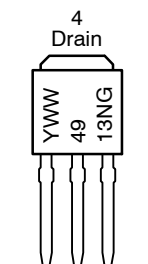
1 Gate 2 Drain 3 Source 4 Drain
