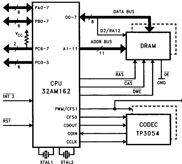
FIGURE 1-1. NS32AM162—Internal ROM Mode
