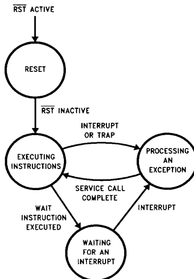
FIGURE 3-1. Operating States
