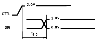
FIGURE 4-2. Synchronous Output Signals Specification
