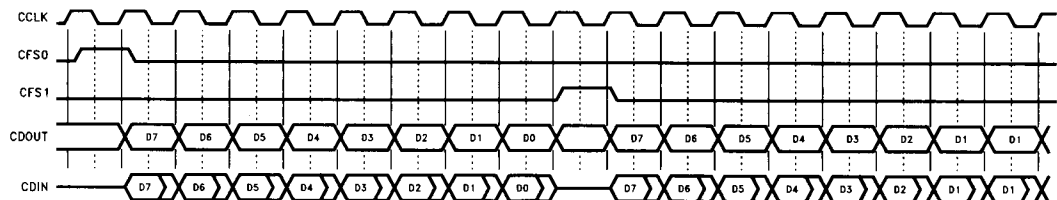
FIGURE 3-6. CODEC Protocol—Short Frame
