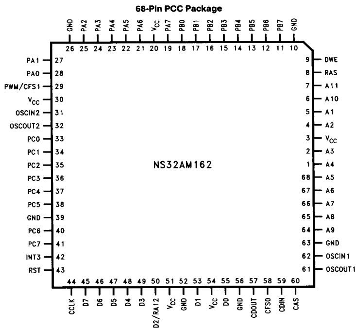
FIGURE 4-1. Connection Diagram
