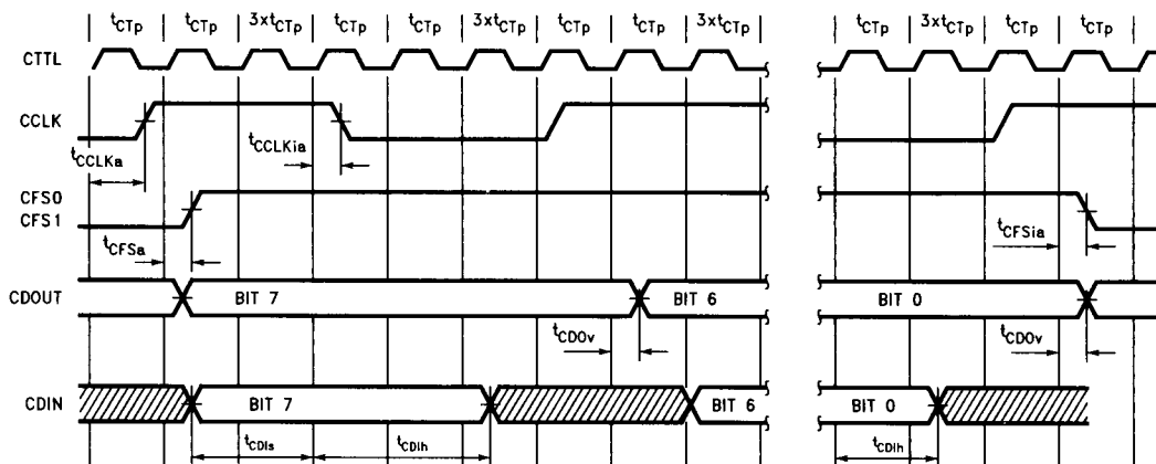
FIGURE 4-8. CODEC Long Frame Timing, 8 KHz Sampling Rate
