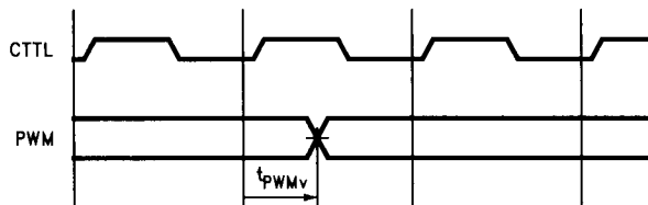
FIGURE 4-13b. PWM Output Timing
