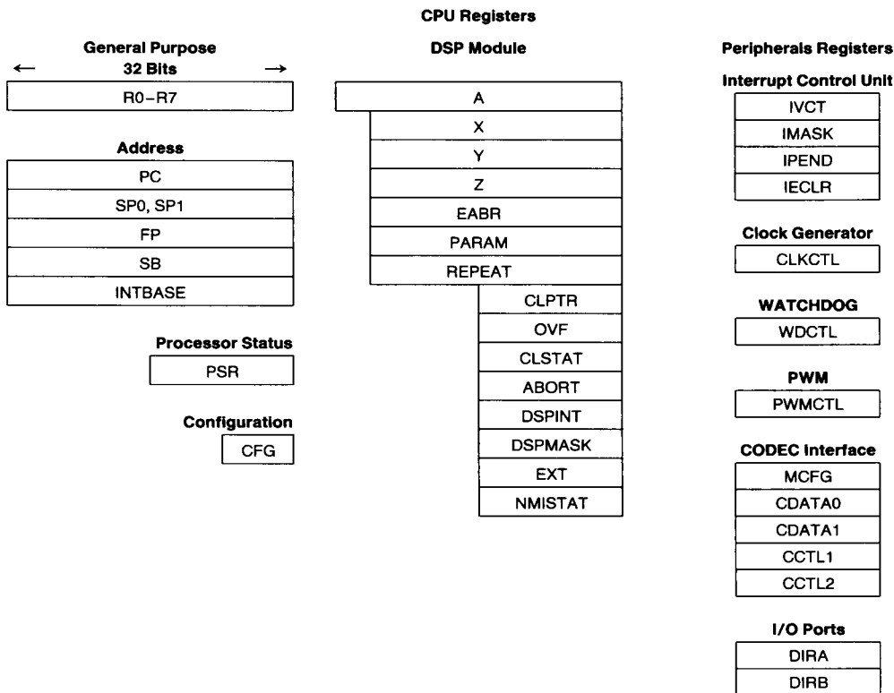
FIGURE 2-1. NS32AM162 Internal Registers
