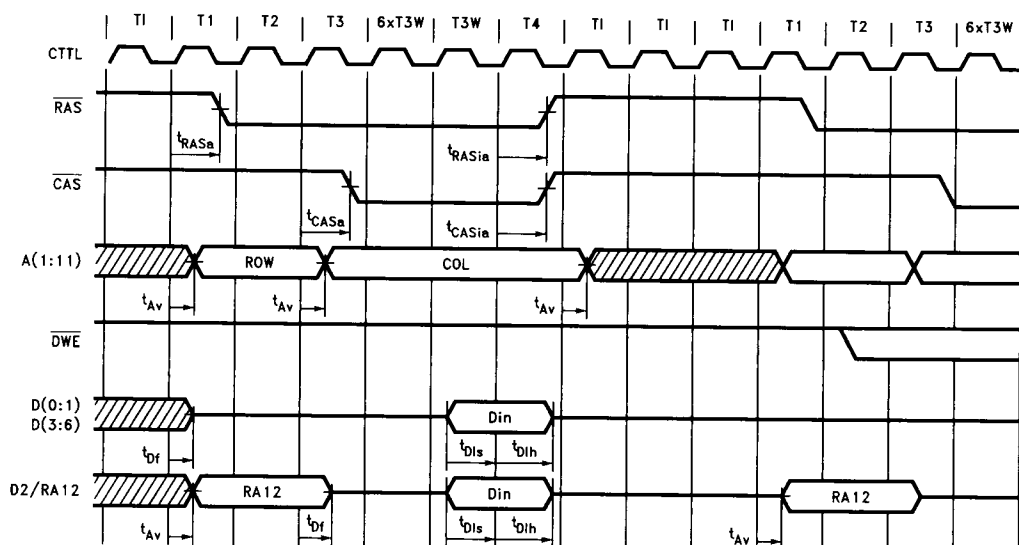
FIGURE 4-5a. DRAM Read Cycle Timing (Internal ROM Mode Only)
