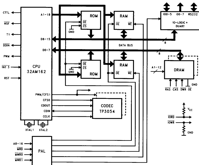
FIGURE 1-3. NS32AM162—Development Mode
