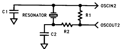
FIGURE 3-10. Low Frequency Resonator Connections
