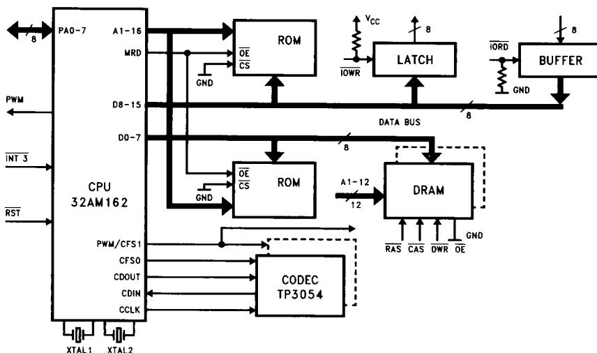
FIGURE 1-2. NS32AM162—External ROM Mode
