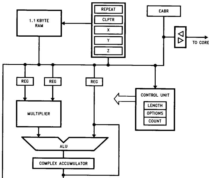
FIGURE 3-8. DSP Module Block Diagram
