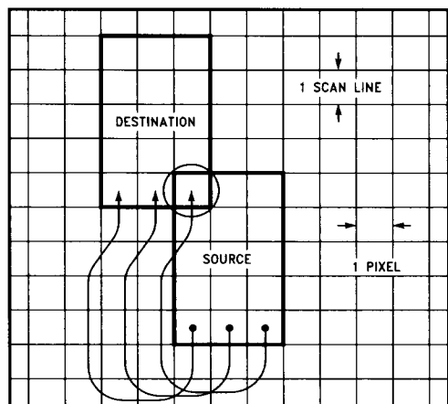
FIGURE 2-26. Overlapping BITBLT Blocks
