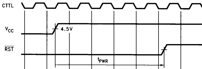
FIGURE 4-17. Power On Reset
