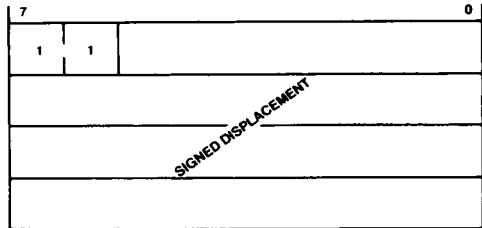
FIGURE 2-23. Displacement Encodings
