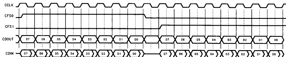
FIGURE 3-7. CODEC Protocol—Long Frame
