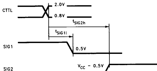
FIGURE 4-4a. PWM Output Signal Specification
