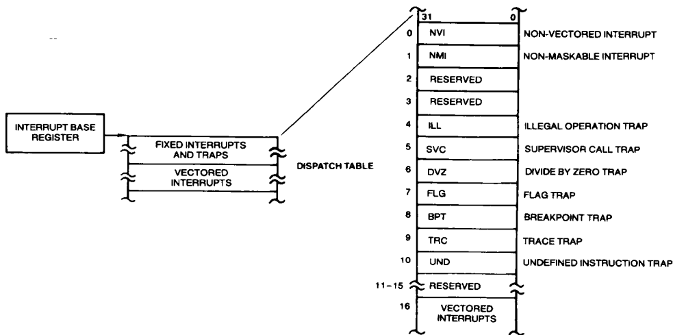
FIGURE 3-2. Interrupt Dispatch and Cascade Tables
