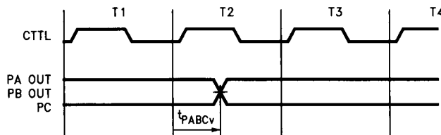
FIGURE 4-13a. Port A, Port B and Port C Timing
