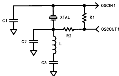
FIGURE 3-9. High Frequency Crystal Connections
