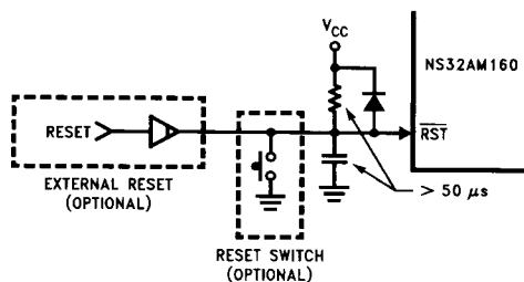
FIGURE 3-11. Recommended Reset Connections
