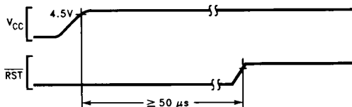
FIGURE 3-12. Power-On Reset Requirements
