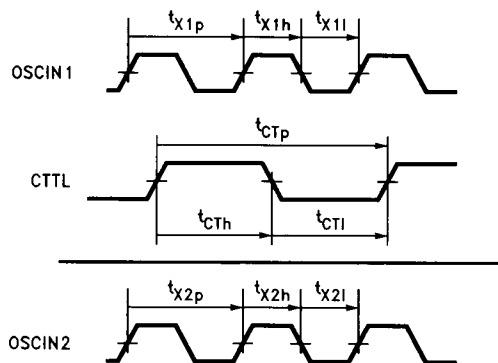
FIGURE 4-15. CCTL, OSCIN1 and OSCIN2 Timing
