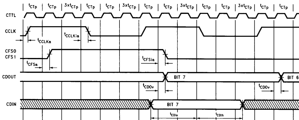
FIGURE 4-9. CODEC Short Frame Timing, 8 KHz Sampling Rate
