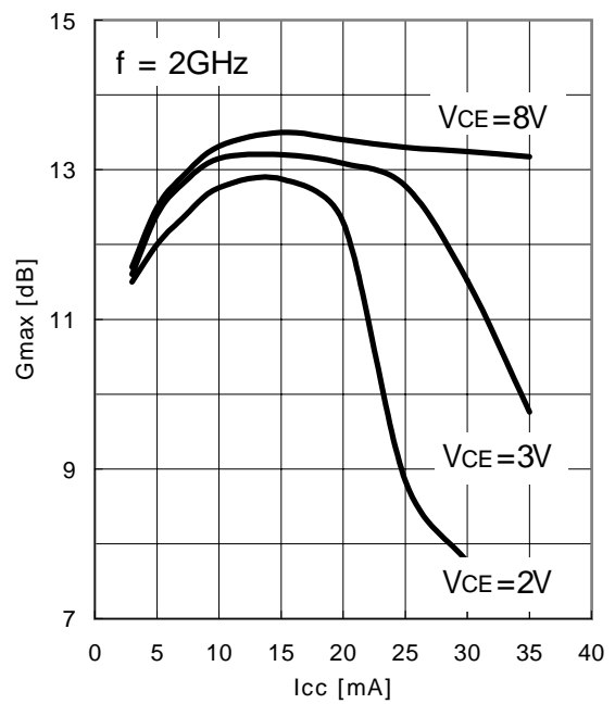
Power Gain : Gmax vs. Icc
