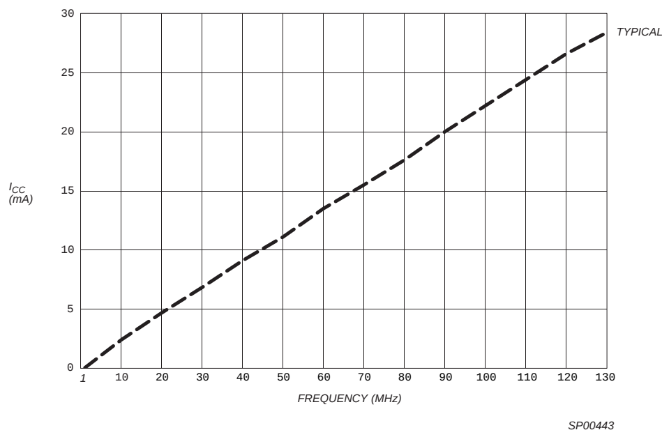
Figure 5: I_{CC} vs. Frequency at V_{CC} = 3.3V , 25^{\circ}C
