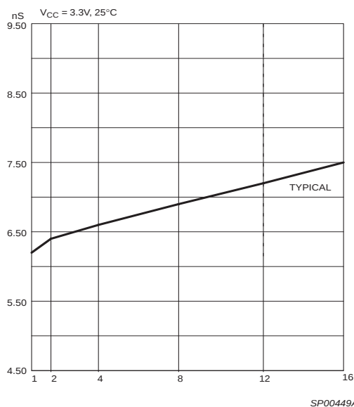
Figure 6: t_{PD\_PAL} vs. Output Switching
