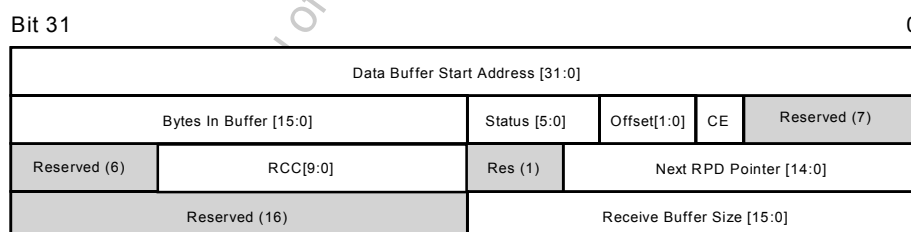
Figure 5 – Receive Packet Descriptor
