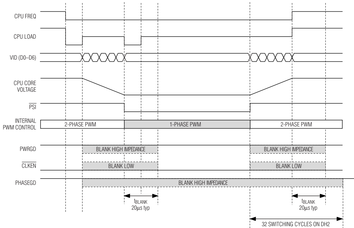
Figure 8. \overline{\text{PSI}} Transition
