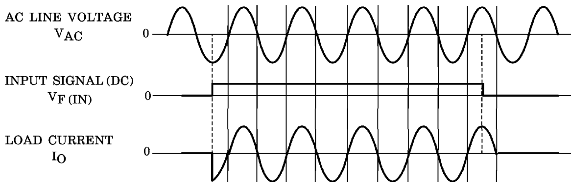
Fig. 1. SWITCHING WAVEFORM
