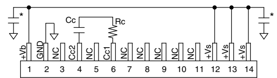
COMPONENT SIDE VIEW
