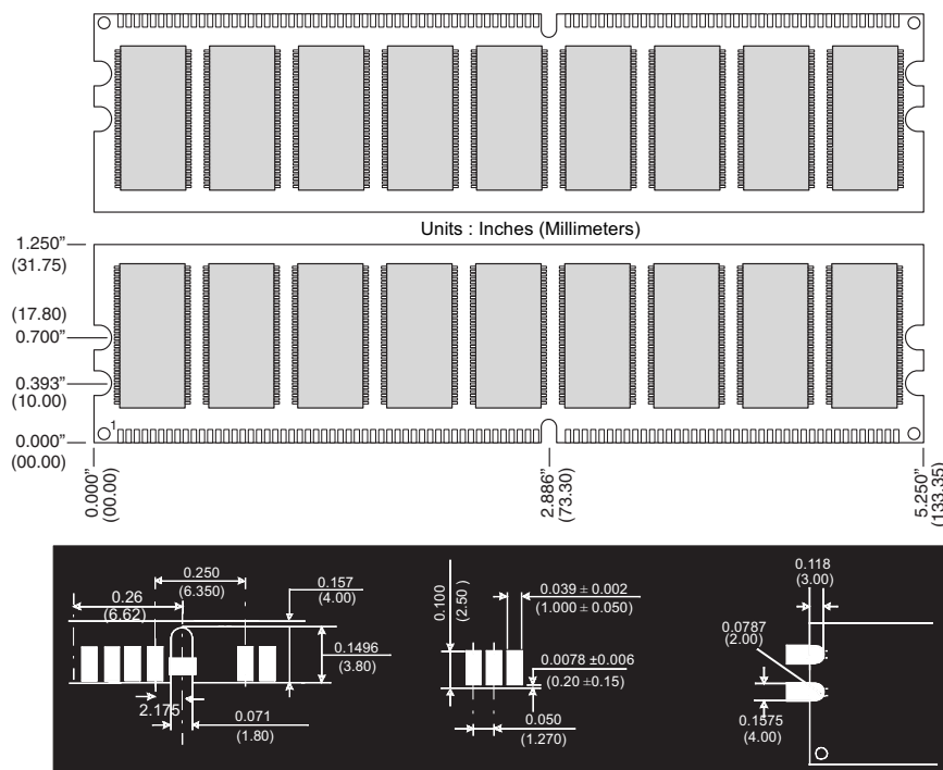
Figure 1: KVR400X72C3A/512 184-Pin DIMM Module
