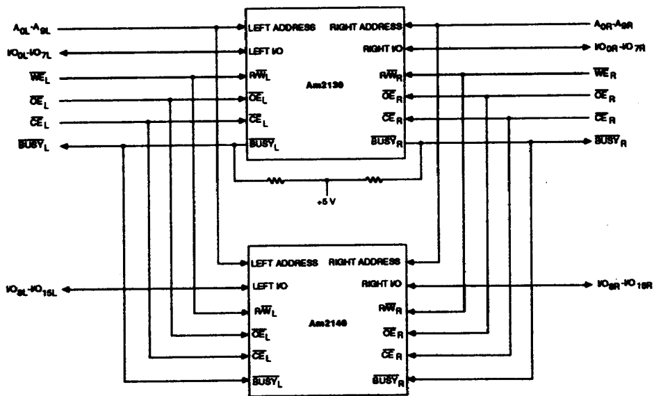
Figure 3. Width Expansion with Master/Slave
