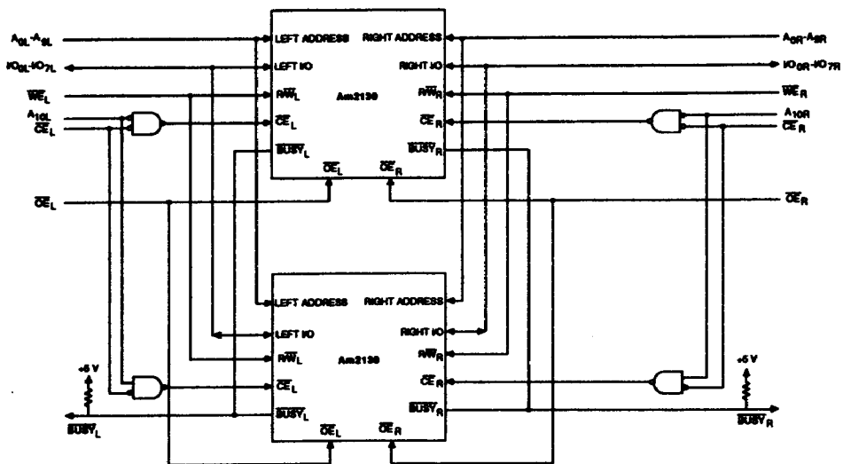
Figure 2. Conceptual Depth Expansion
