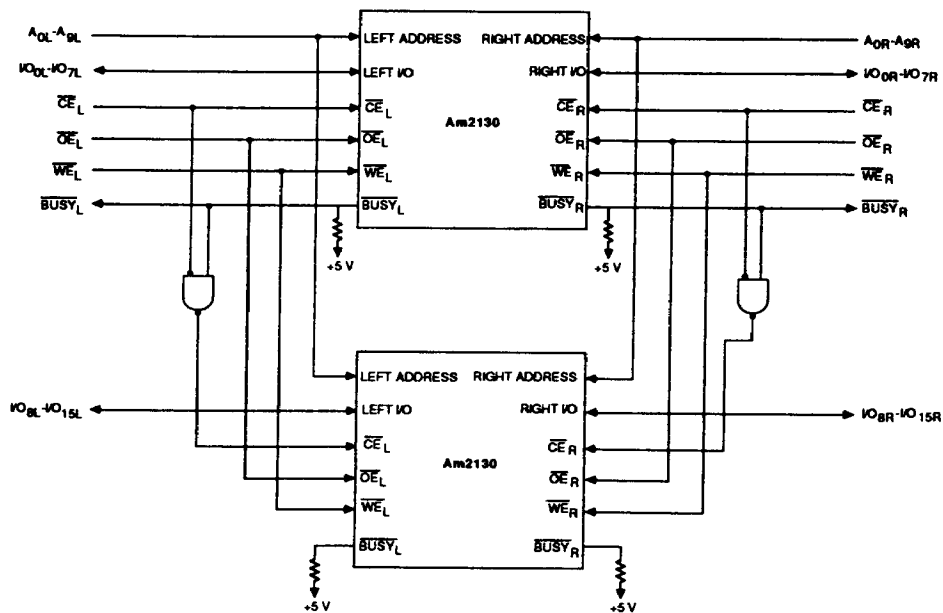
Figure 4. Width Expansion with Master
