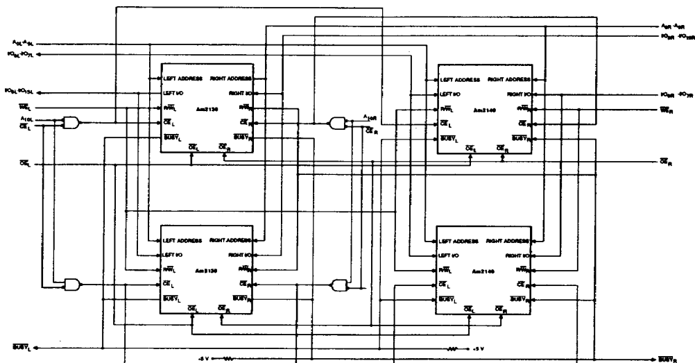
Figure 5. Conceptual Diagram of a 2K x 16 System Using Master/Slave
