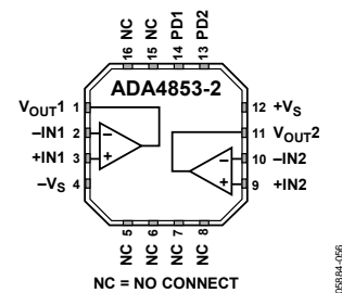
Figure 2. 16-Lead LFCSP_VQ
