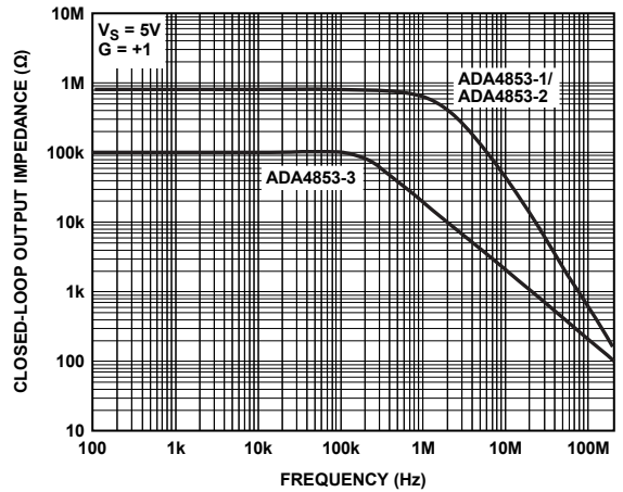
Figure 22. Output Impedance vs. Frequency Disabled
