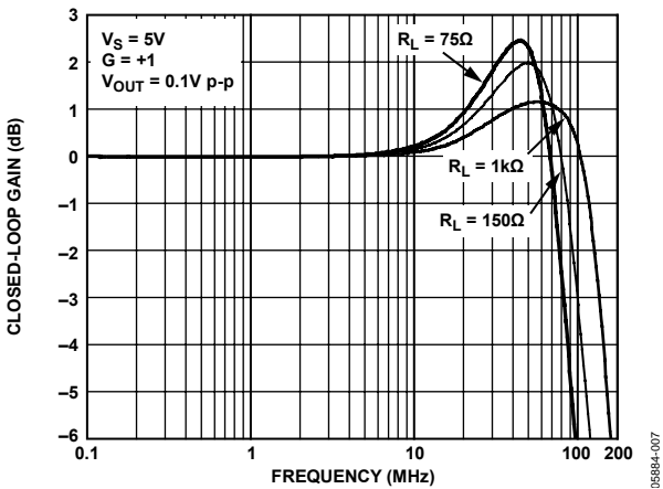
Figure 8. Small Signal Frequency Response for Various Loads
