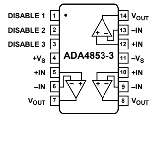
Figure 4. 16-Lead TSSOP
