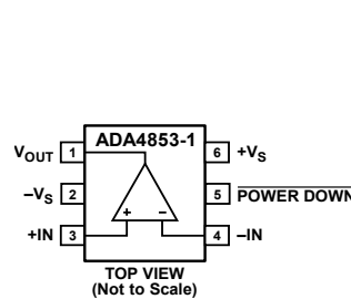
Figure 1. 6-Lead SC70
