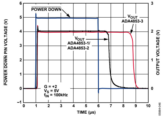
Figure 47. Enable/Disable Time
