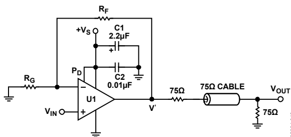
Figure 51. Video Amplifier
