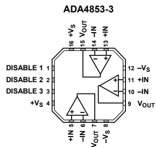
Figure 3. 16-Lead LFCSP_VQ
