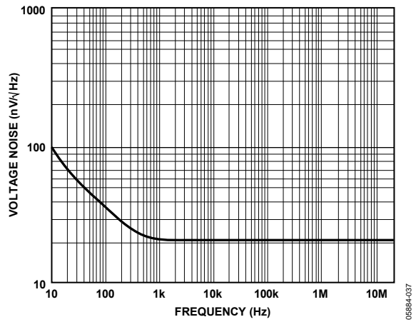
Figure 34. Voltage Noise vs. Frequency
