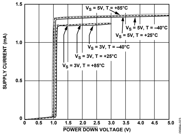
Figure 38. Supply Current vs. \overline{\text{POWER DOWN}} Voltage
