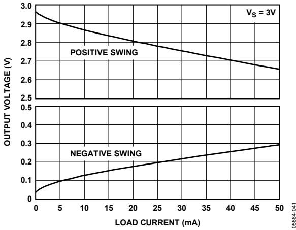
Figure 43. Output Voltage vs. Load Current
