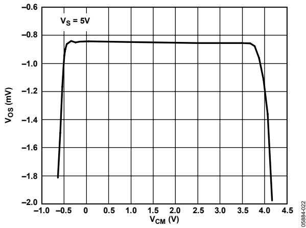
Figure 37. V_{os} vs. Common-Mode Voltage
