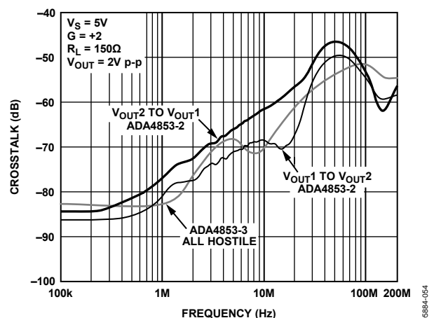
Figure 48. Crosstalk vs. Frequency
