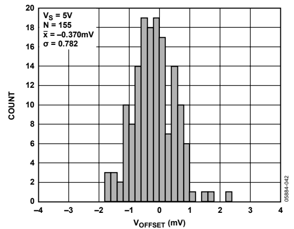
Figure 36. V_{0S} Distribution
