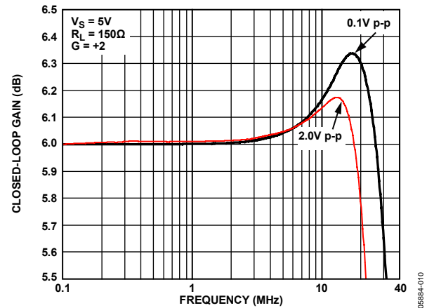
Figure 11. 0.5 dB Flatness Response for Various Output Voltages
