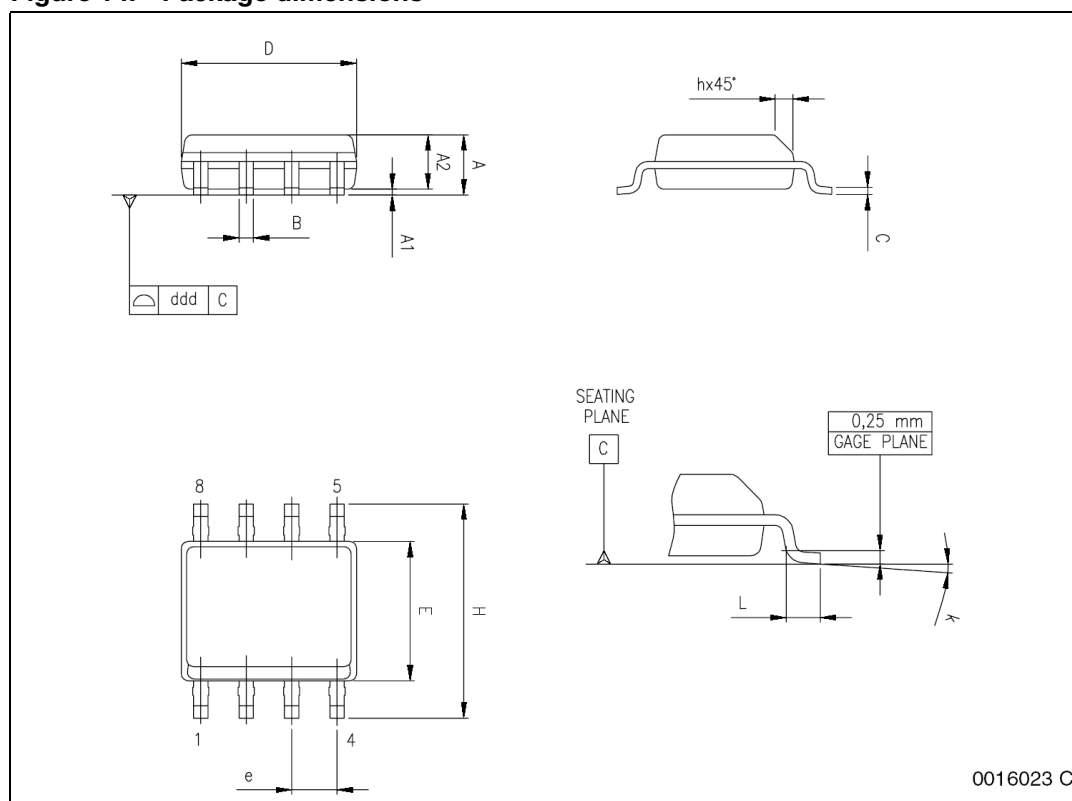
Figure 14. Package dimensions
