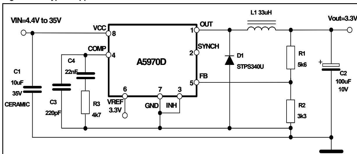
Figure 1. Typical application
