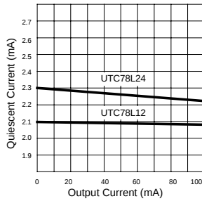
Fig.7 UTC78L12/24 quiescent current vs output current ( T_j=25^{\circ}C )
