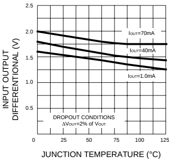
Fig.10 Dropout Voltage
