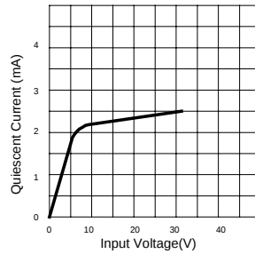
Fig.8 UTC78L05 Quiescent Current vs. Input Voltage ( I_o=0mA, T_j=25^{\circ}C )
