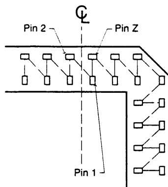
44 LEAD PLCC
