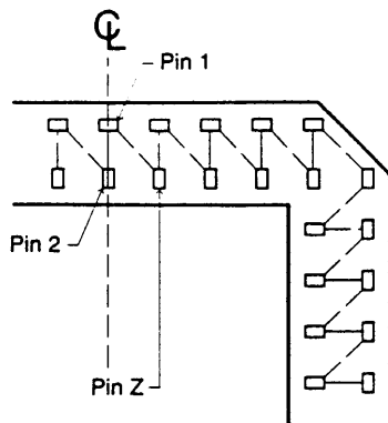
20, 28, 32, 52, 68 & 84 LEAD PLCC
