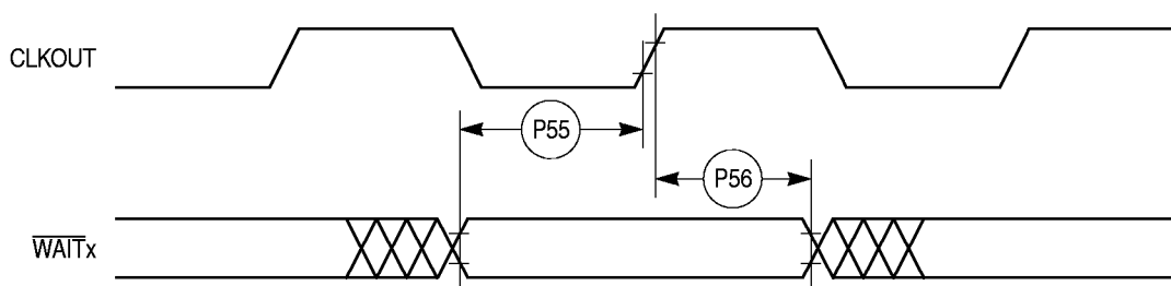
Figure 25. PCMCIA \overline{WAIT} Signals Detection Timing
