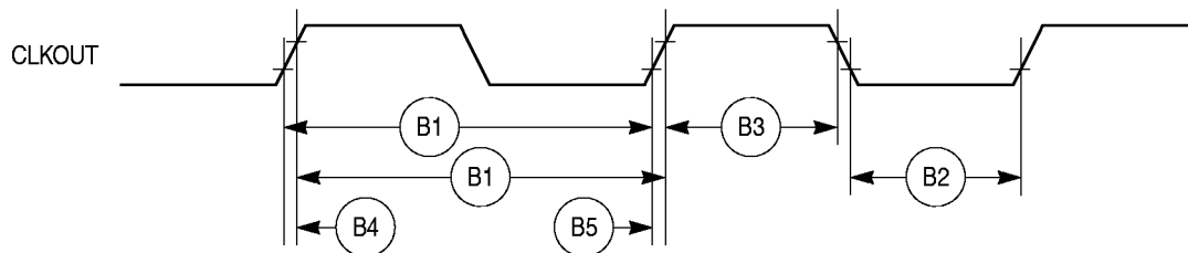
Figure 2. External Clock Timing
