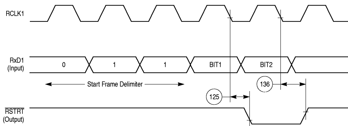
Figure 59. CAM Interface Receive Start Timing Diagram
