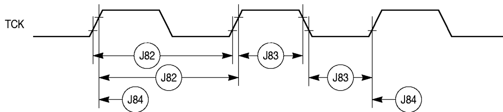
Figure 33. JTAG Test Clock Input Timing
