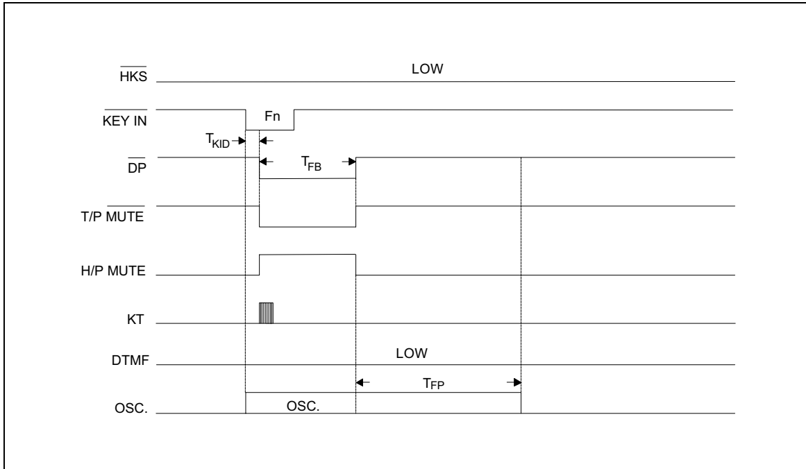
Figure 8. Flash Operation Timing Diagram
