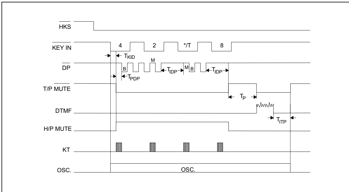
Figure 7(a). Pulse to Tone Function Timing Diagram
