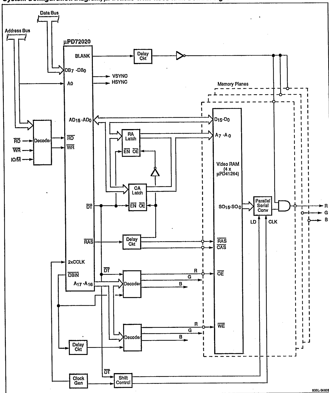
System Configuration Diagram; \mu PD72020 With Video RAM Control Signal \overline{DT}
