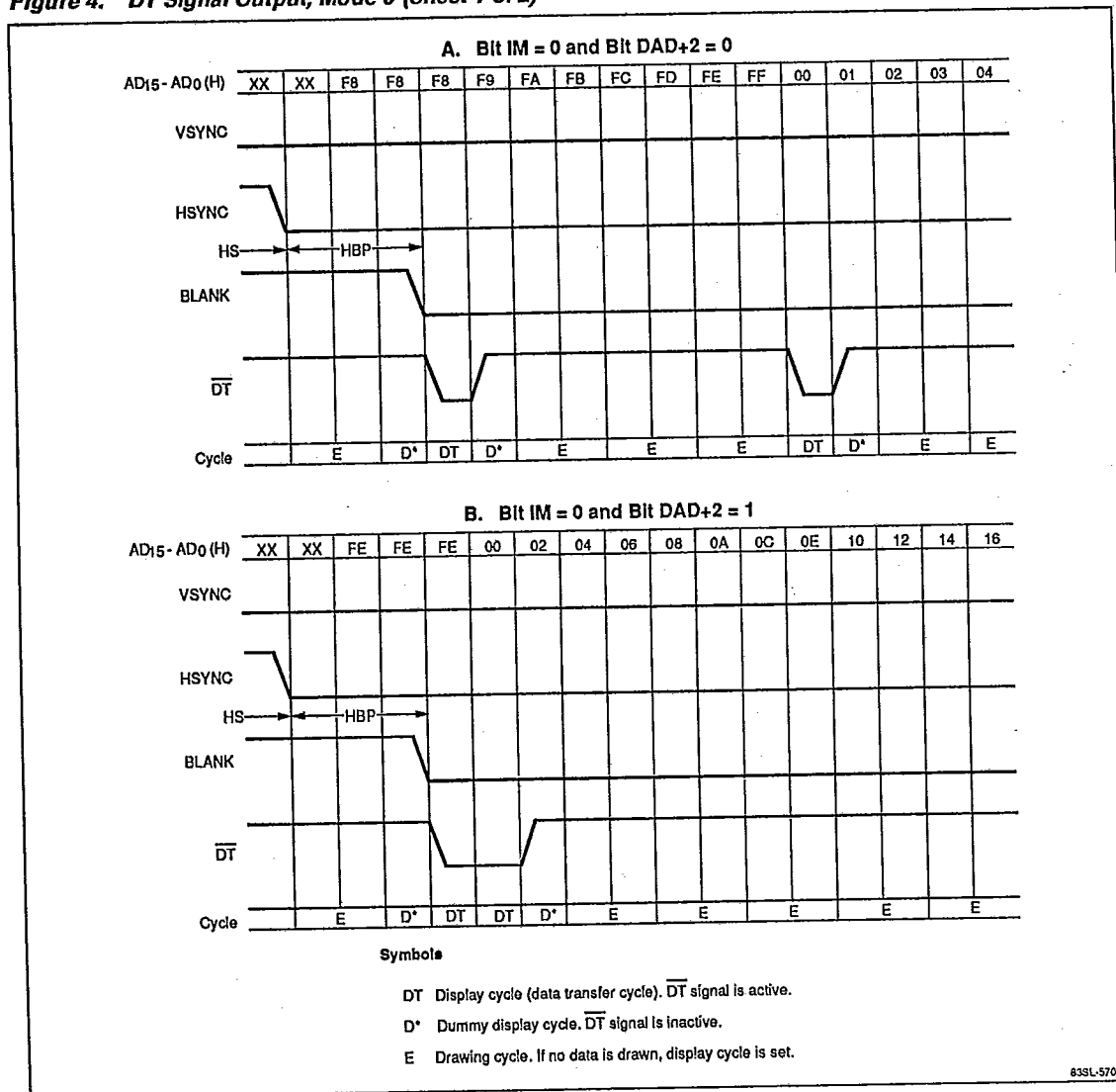
Figure 4. \overline{DT} Signal Output, Mode 0 (Sheet 1 of 2)
