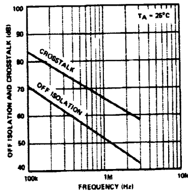
CROSSTALK AND "OFF" ISOLATION vs FREQUENCY
