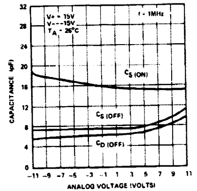
SWITCH CAPACITANCE vs ANALOG VOLTAGE
