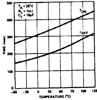
SWITCHING TIME vs TEMPERATURE
