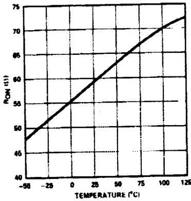
RON vs TEMPERATURE
