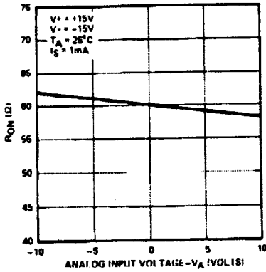
"ON" RESISTANCE vs ANALOG VOLTAGE ( V_A )
