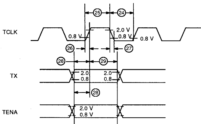
TCLK and TX Timing
