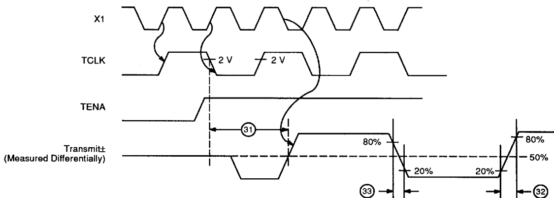
Transmit Timing (at start of packet)
