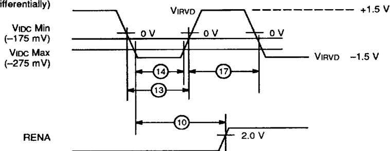
Receive± Input Pulse Width Timing
