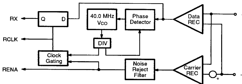
Figure 5. Receiver Section Detail
