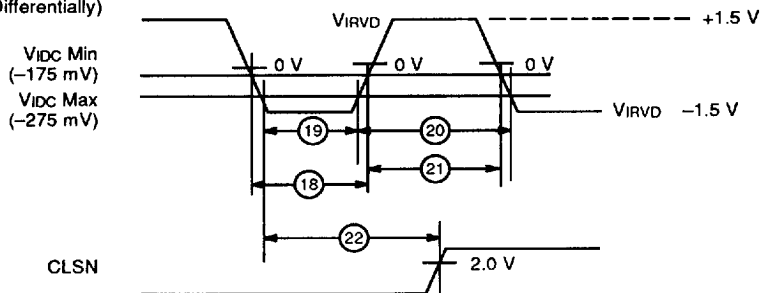
Collision± Input Pulse Width Timing
