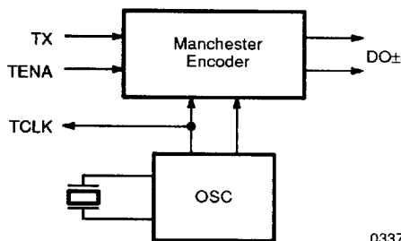
Figure 1. Transmit Section
