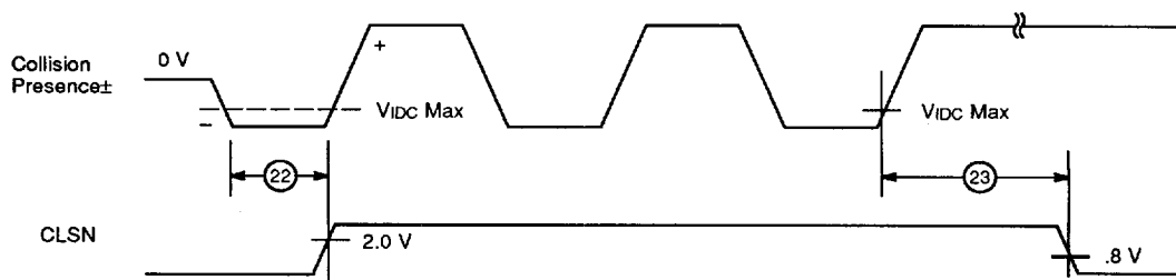
Collision Timing
