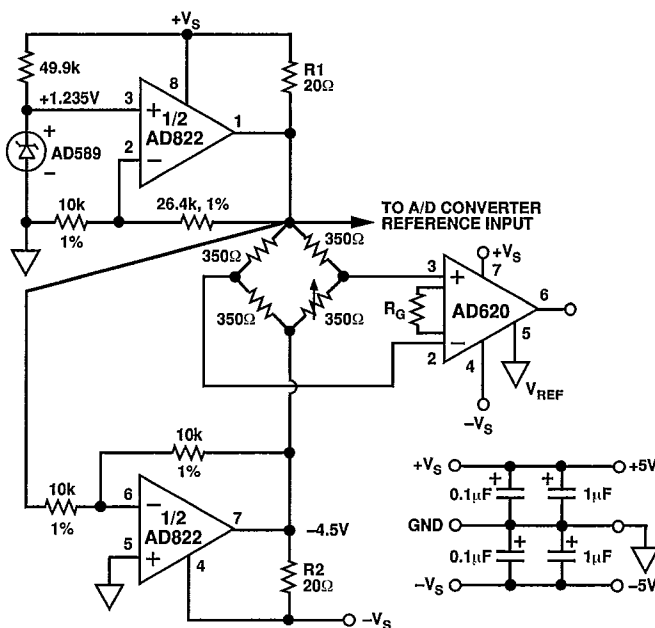
Figure 47. Low Dropout Bipolar Bridge Driver
