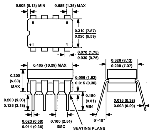
Cerdip (Q) Package
