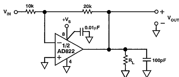
Figure 33. Gain of Two Inverter
