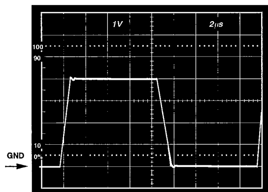
Figure 31. V_S = +5\text{ V}, 0\text{ V} ; Unity Gain Follower Response to 0 V to 4 V Step
