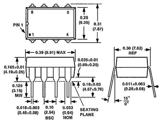
Mini-DIP (N) Package
