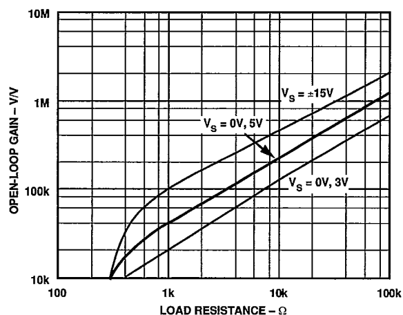
Figure 7. Open-Loop Gain vs. Load Resistance
