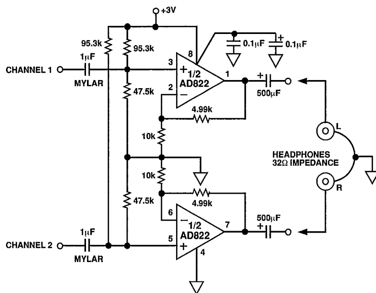
Figure 46. 3 Volt Single Supply Stereo Headphone Driver
