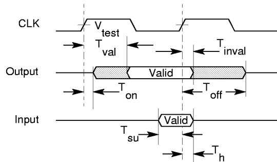
Figure 15–2 PCI Signal Timing Measurement Conditions
