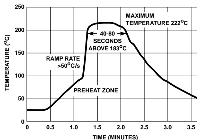
FIGURE 13. VAPOR PHASE SOLDER PROFILE
