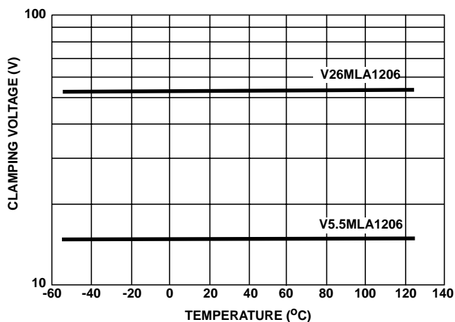
FIGURE 9. CLAMPING VOLTAGE OVER TEMPERATURE (V C AT 10A)
