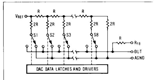
Figure 1. Simplified DAC Schematic
