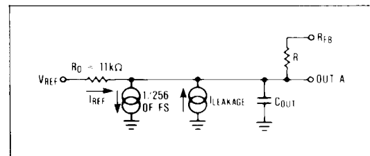
Figure 2. DAC Equivalent Circuit. All Digital Inputs High
