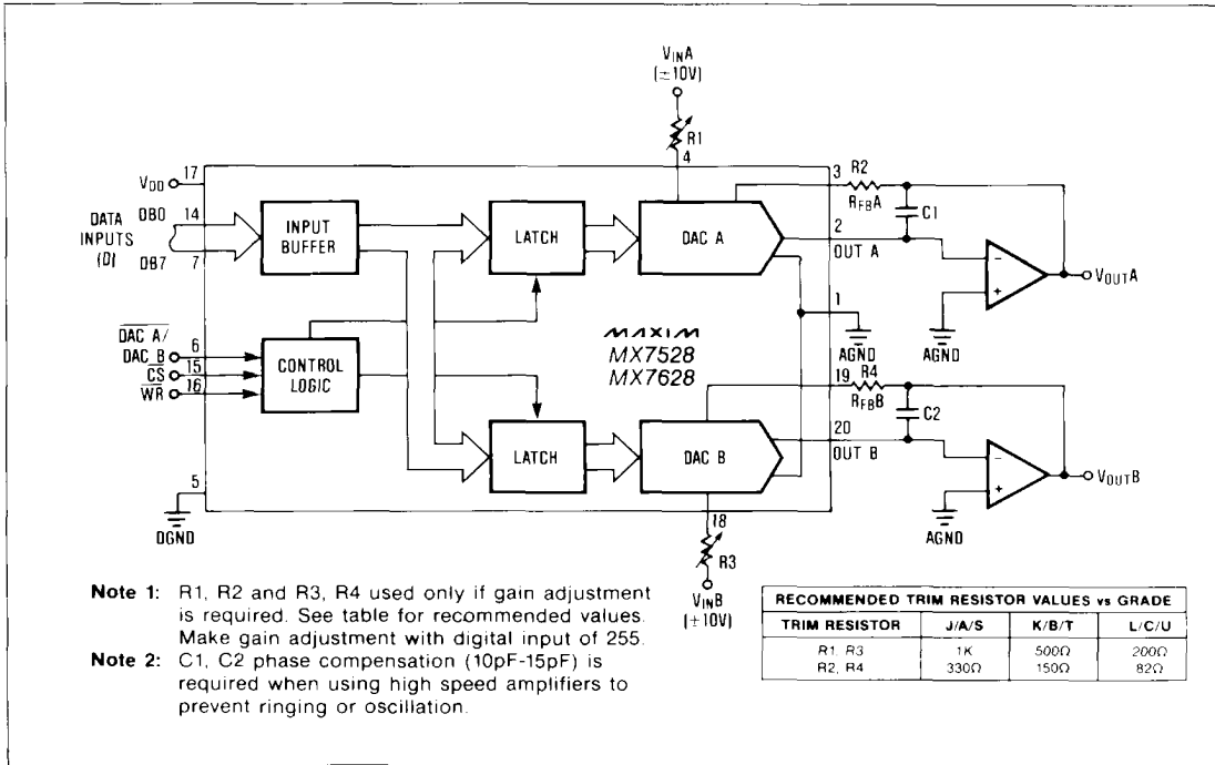
Figure 4. Dual DAC Unipolar Binary Operation (2 Quadrant Multiplication)
