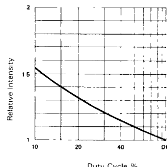
Duty Cycle % Fig. 6 LUMINOUS INTENSITY VS DUTY CYCLE % (AVERAGE I_F = 10 \text{ mA PER SEG} )
