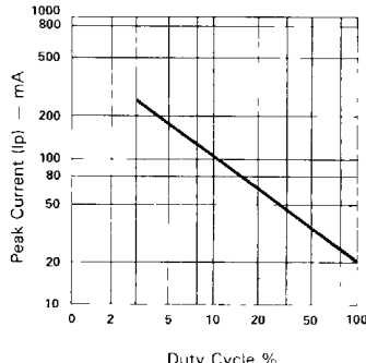
Duty Cycle % Fig. 5 MAX PEAK CURRENT VS DUTY CYCLE % (REFRESH RATE — F = 1 \text{ KHz} )
