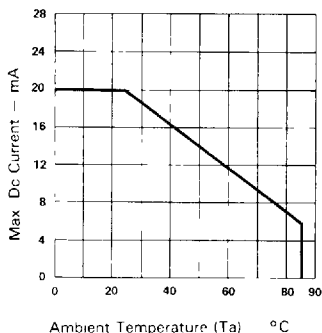
Ambient Temperature ( T_A ) — ^\circ\text{C} Fig. 4 MAX ALLOWABLE DC CURRENT PER SEG VS AMBIENT TEMPERATURE
