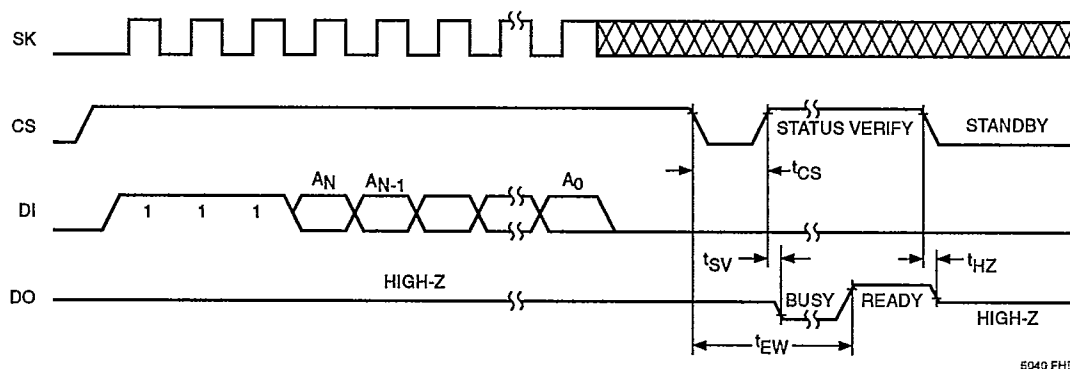
Figure 4. Erase Instruction Timing
