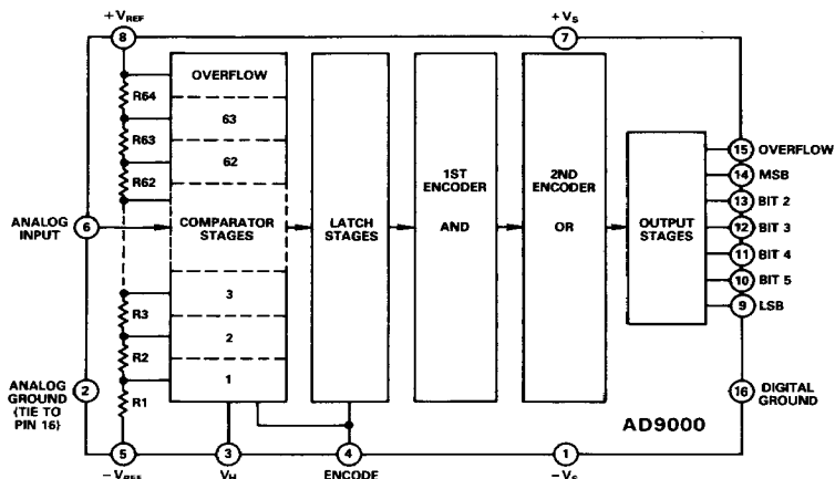
AD9000 Functional Block Diagram
