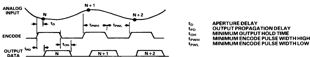
System Timing Diagram
