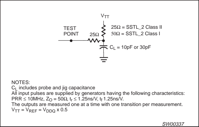
Figure 1. Load circuitry
