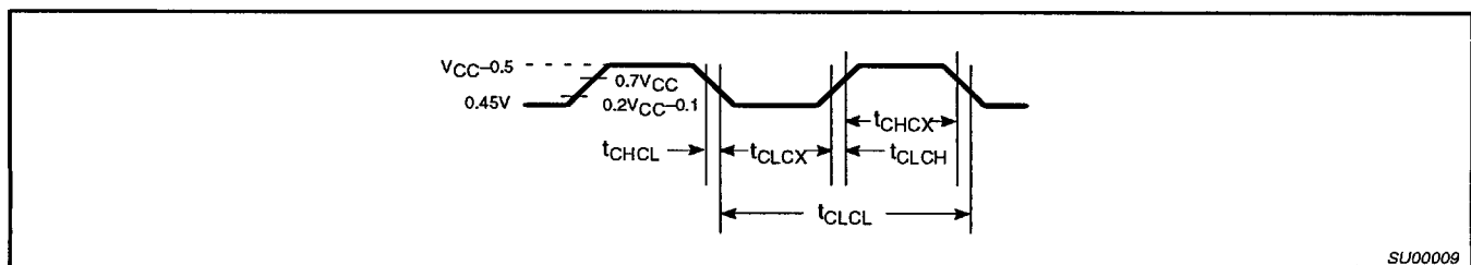
Figure 8. External Clock Drive
