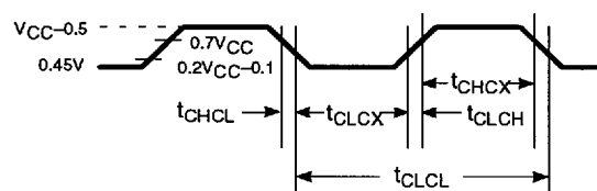
Figure 14. Clock Signal Waveform for I_{CC} Tests in Active and Idle Modes t_{CLCH} = t_{CHCL} = 5\text{ns}
