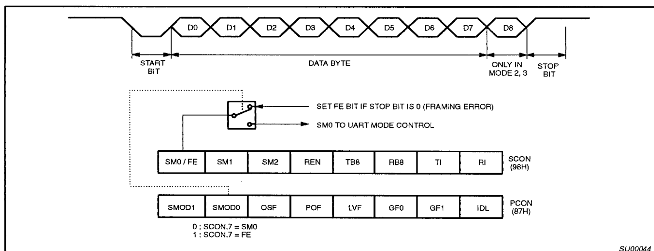
Figure 2. UART Framing Error Detection
