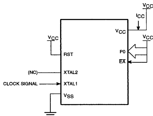
Figure 12. I_{CC} Test Condition, Active Mode All other pins are disconnected
