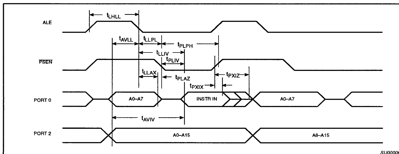
Figure 4. External Program Memory Read Cycle
