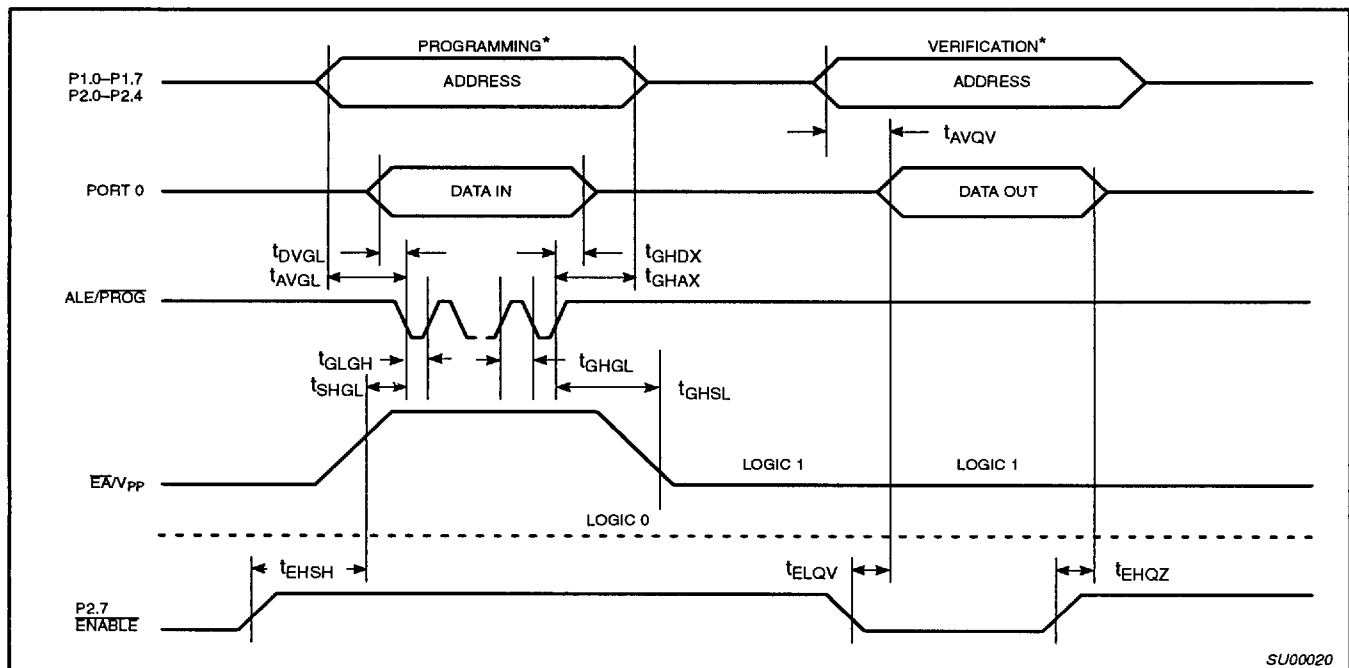
Figure 19. EPROM Programming and Verification
