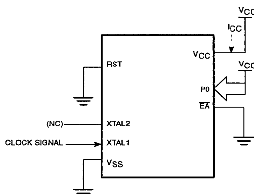
Figure 13. I_{CC} Test Condition, Idle Mode All other pins are disconnected
