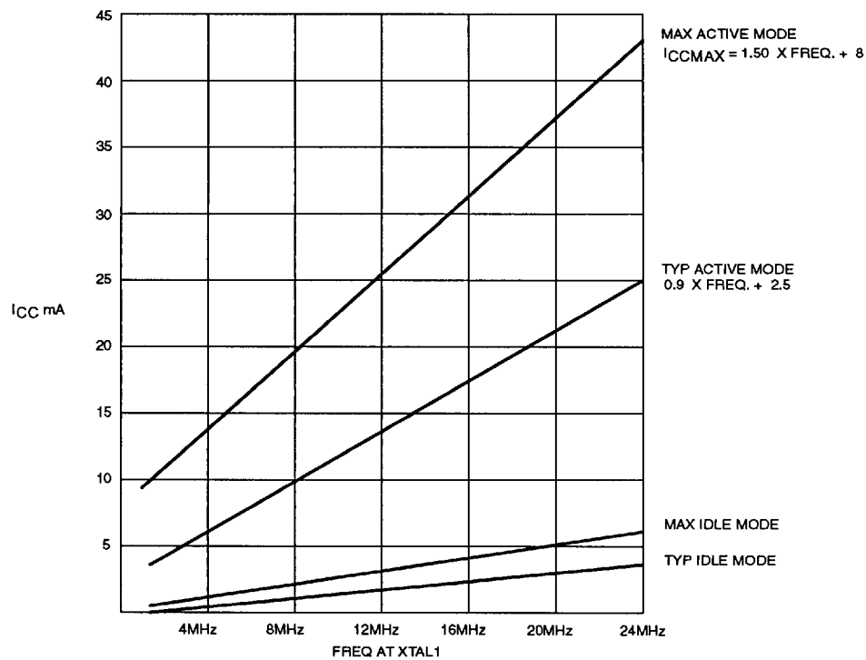
Figure 11. I_{CC} vs. FREQ Valid only within frequency specifications of the device under test
