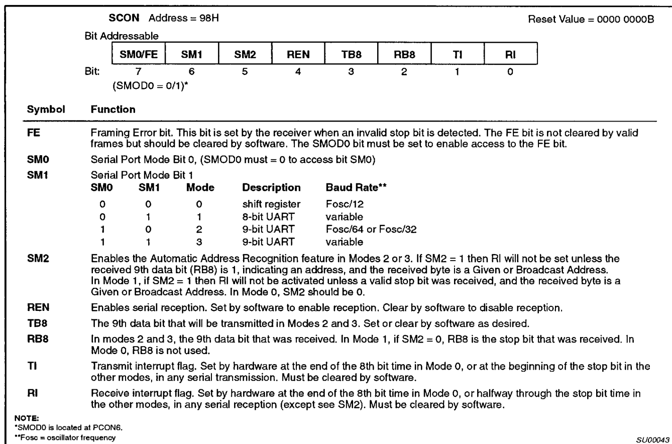
Figure 1. SCON: Serial Port Control Register
