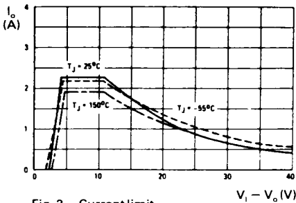
Fig. 2 Current limit
