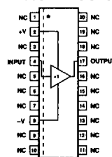
EL2003 M Package
