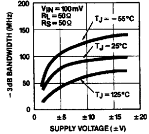
-3 dB Bandwidth vs Supply Voltage
