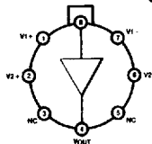
EL2003 H Package
