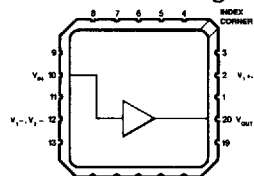
EL2003 M Package
