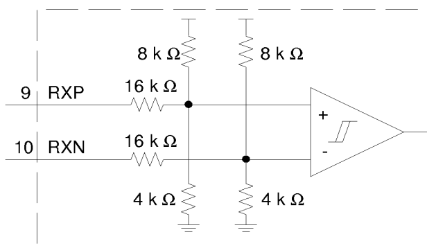
Figure 20. RS422 Receiver Internal Circuit
