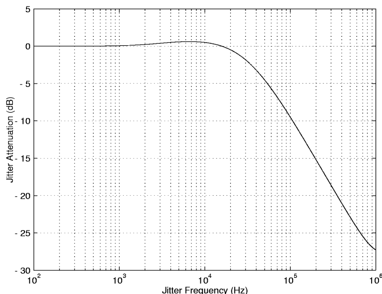
Figure 3. Jitter Attenuator Characteristics
