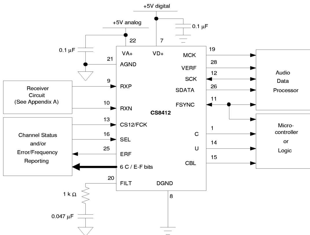
Figure 2. CS8412 Typical Connection Diagram
