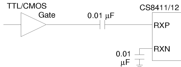
Figure 24. TTL/CMOS Interface
