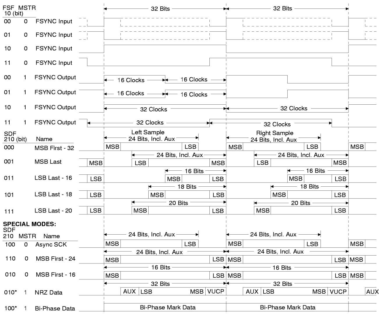
Figure 10. CS8411 Serial Port SDATA and FSYNC Timing
