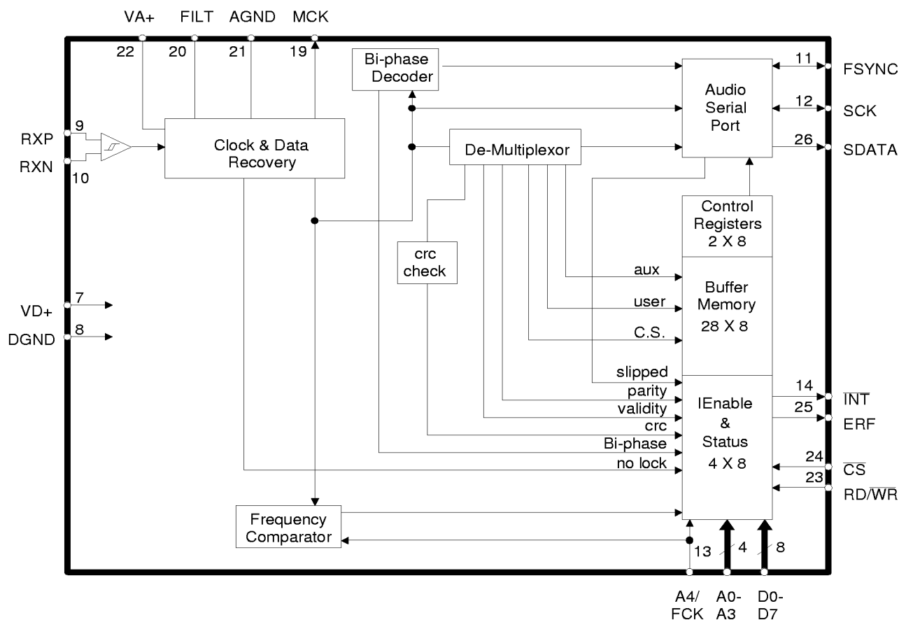
Figure 4. CS8411 Block Diagram
