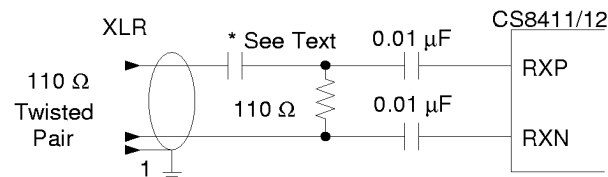
Figure 22. Transformerless Professional Circuit
