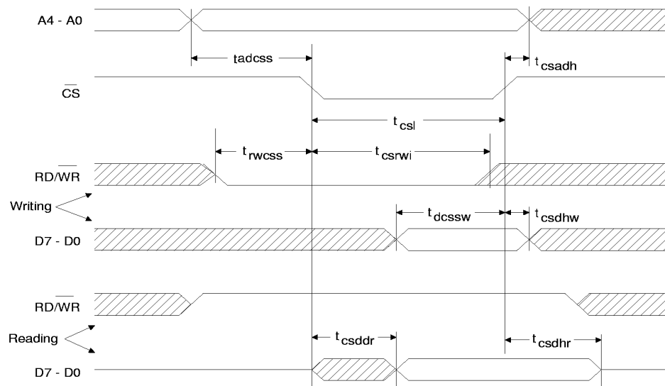
CS8411 Parallel Port Timing
