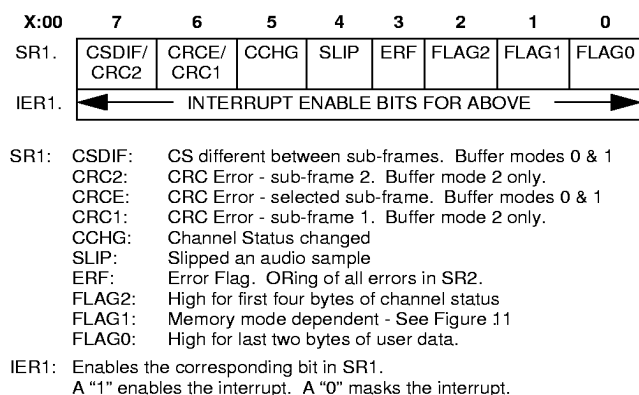
Figure 6. Status/IEnable Register 1
