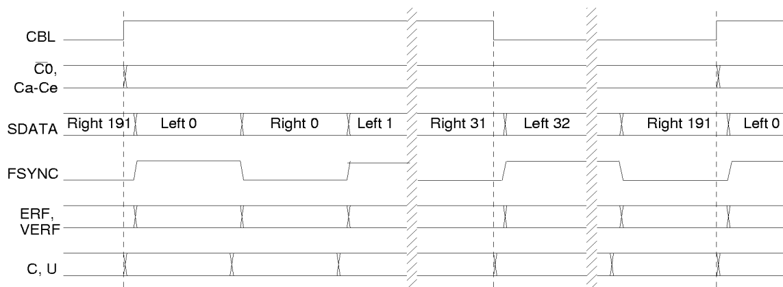
Figure 19. CBL Timing
