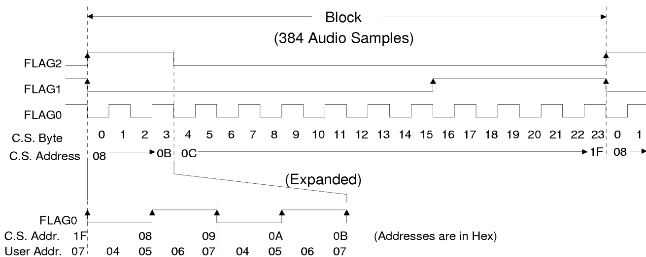
Figure 12. CS8411 Buffer Memory Write Sequence - MODE 0
