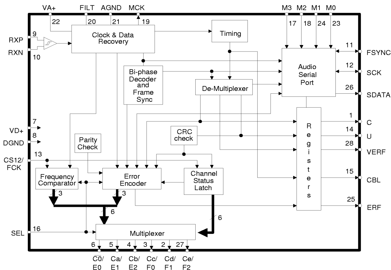
Figure 16. CS8412 Block Diagram
