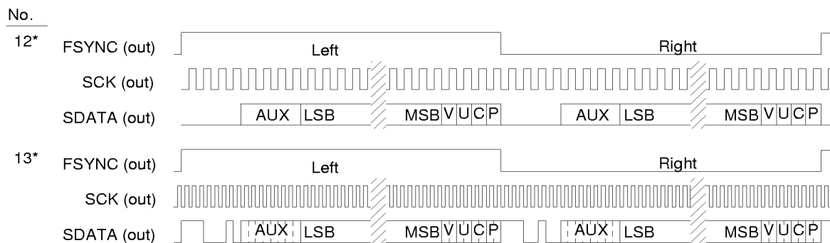
Figure 18. Special Audio Port Formats 12 and 13
