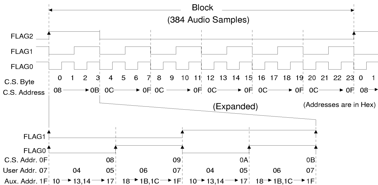
Figure 13. CS8411 Buffer Memory Write Sequence - MODE 1
