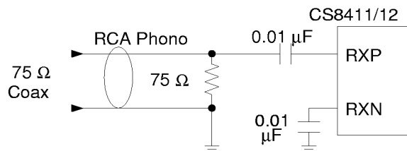
Figure 23. Consumer Input Circuit
