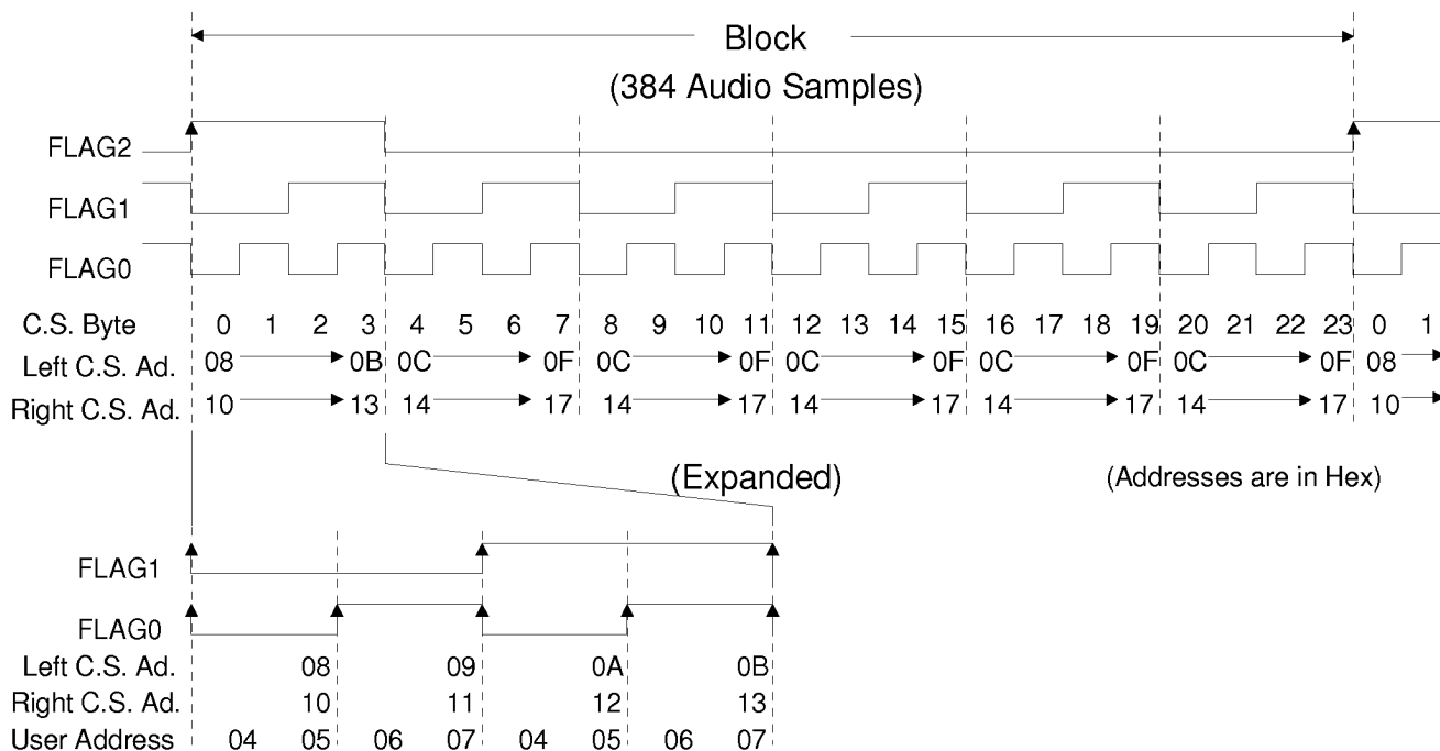
Figure 14. CS8411 Buffer Memory Write Sequence - MODE 2
