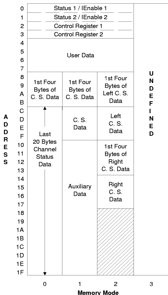
Figure 5. CS8411 Buffer Memory Map
