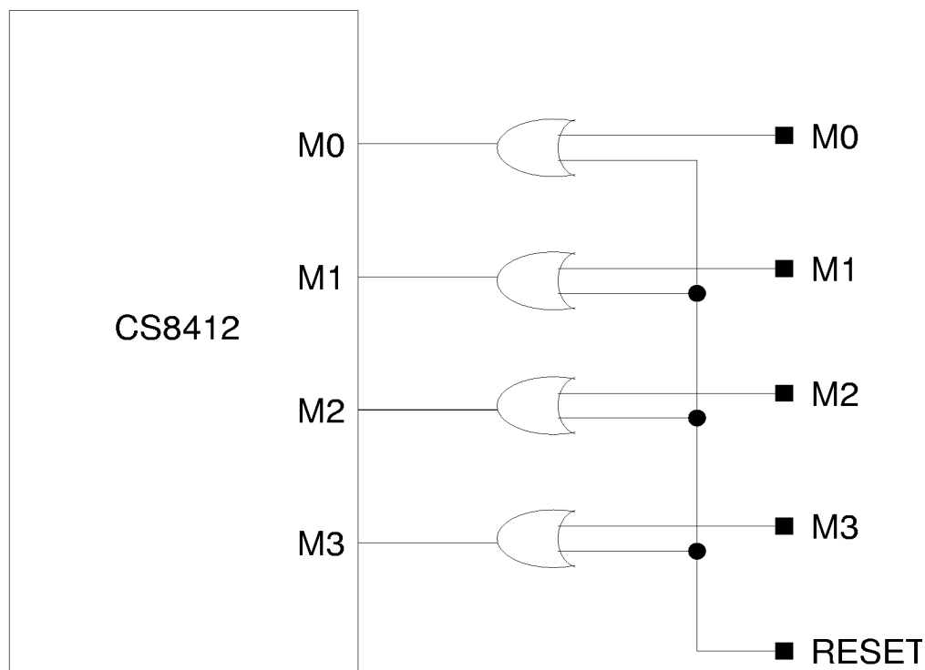
Figure 25. CS8412 Reset Circuit
