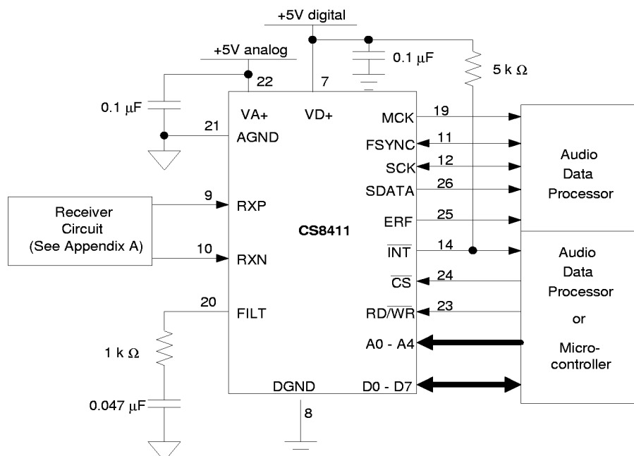
Figure 1. CS8411 Typical Connection Diagram
