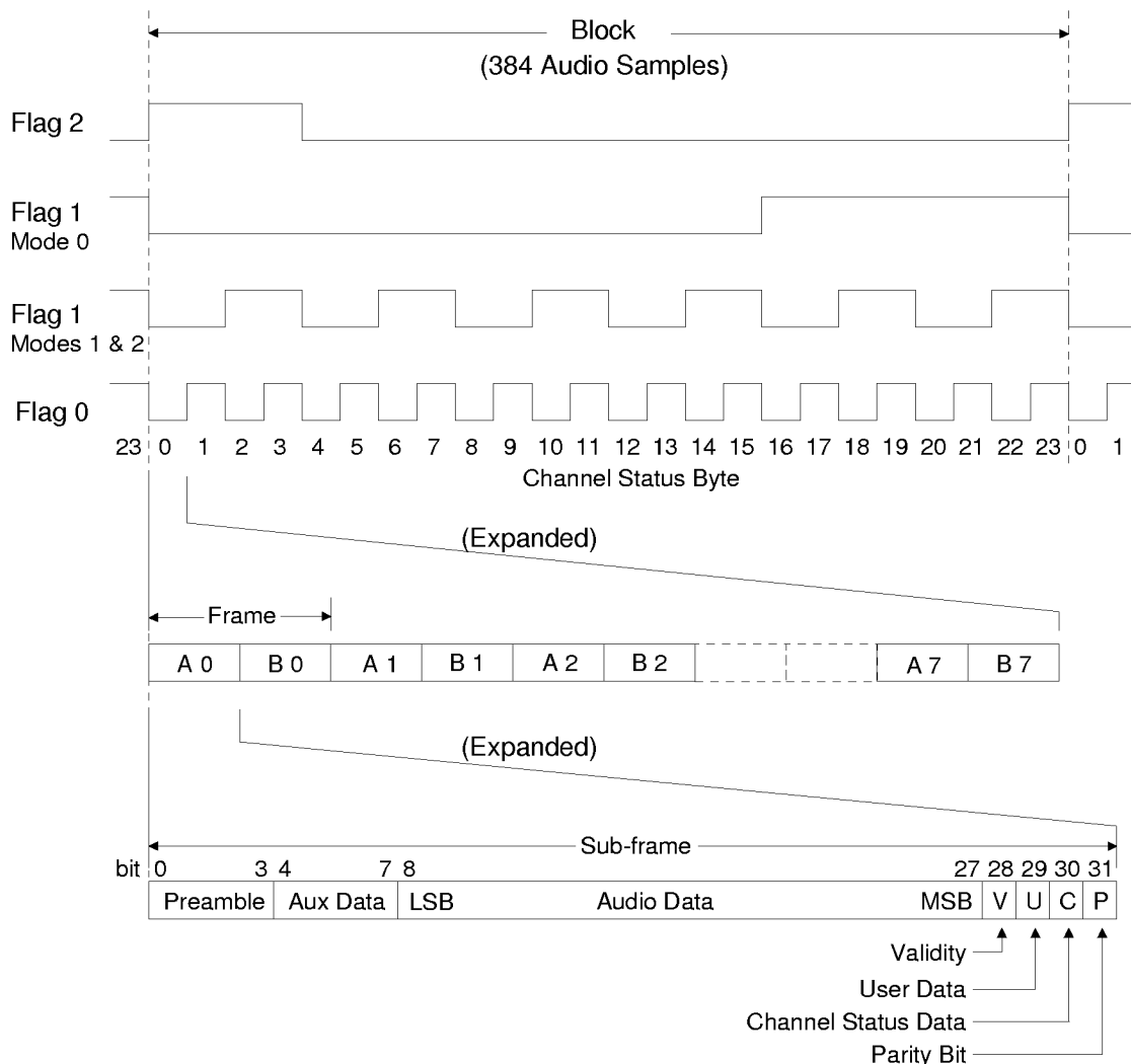
Figure 11. CS8411 Status Register Flag Timing
