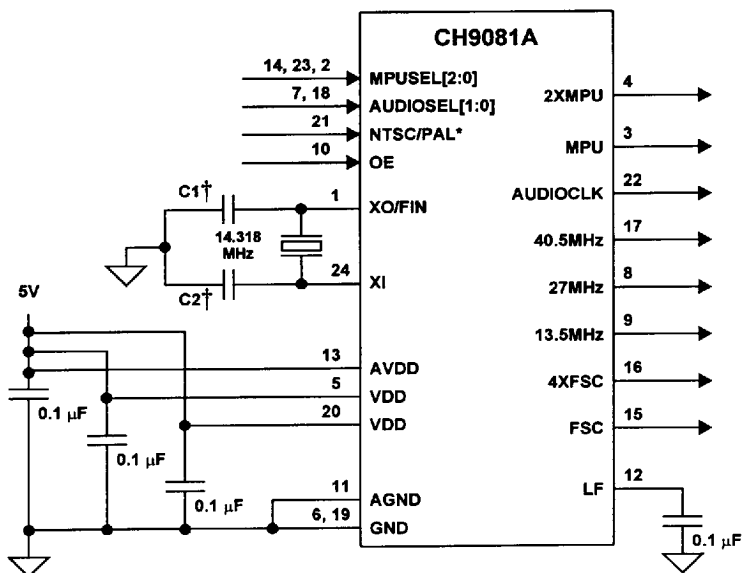
Figure 3: Application Schematic
