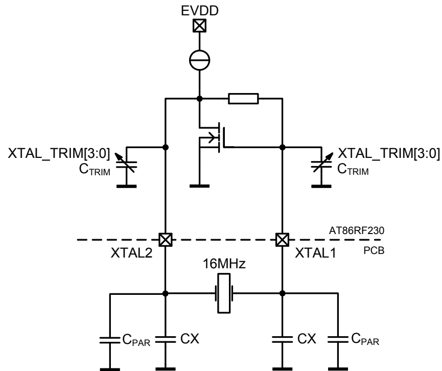
Figure 9-4. Simplified XOSC Schematic with External Components
