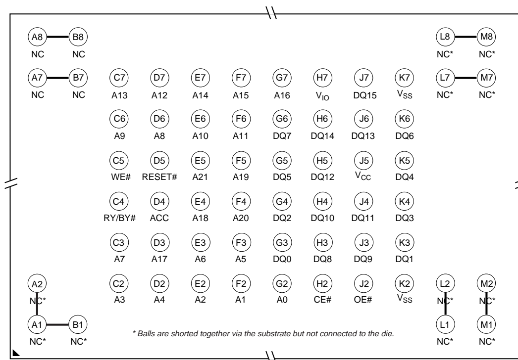
Figure 1. Fine-Pitch BGA Package (63-ball) Connection Diagram
