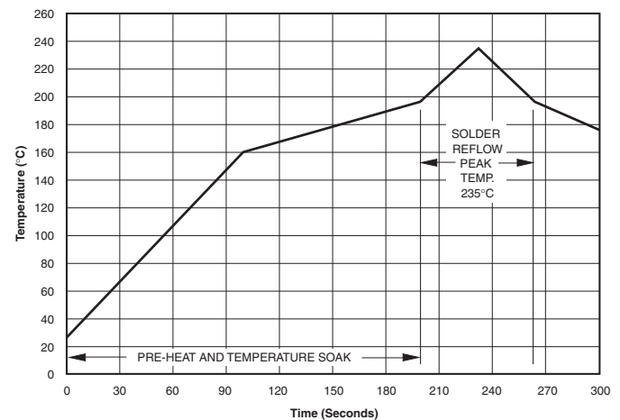
Figure 6. Optimal Solder Reflow Profile
