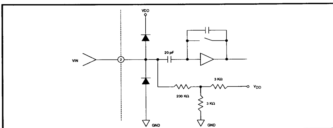
FIGURE 1: VIN Equivalent Input Circuit
