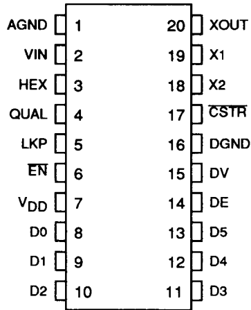
20 - PIN DIP
