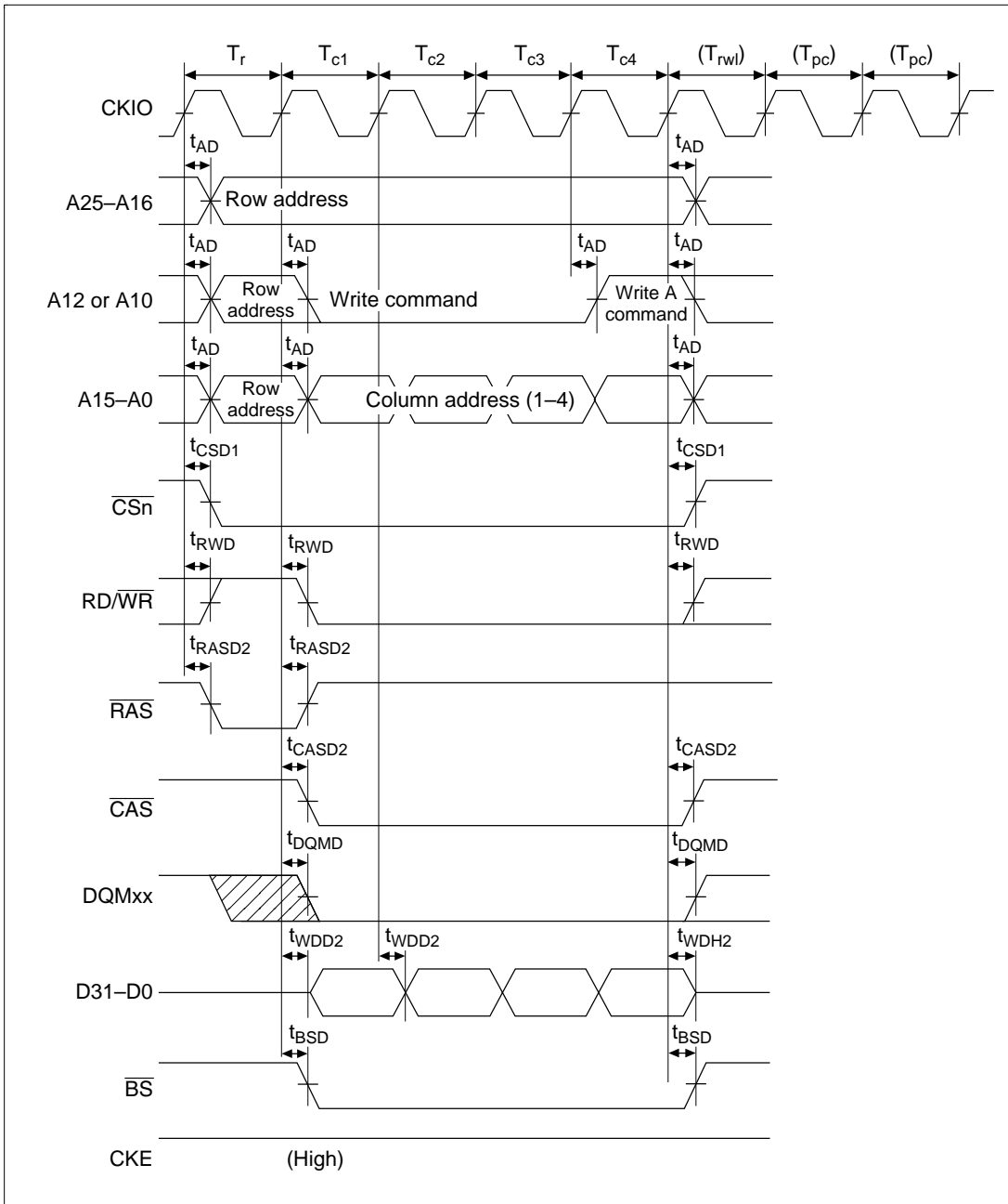
Figure 16.40 Synchronous DRAM Write Bus Cycle (Burst Mode (Single Write \times 4), RCD = 0, TPC = 1, TRWL = 0)
