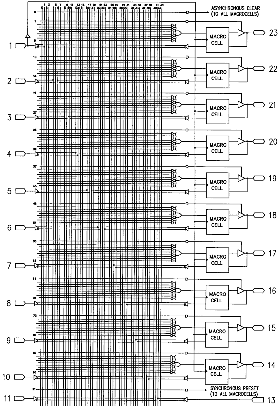
Figure 3. PEEL20CG10 Logic Array Diagram
