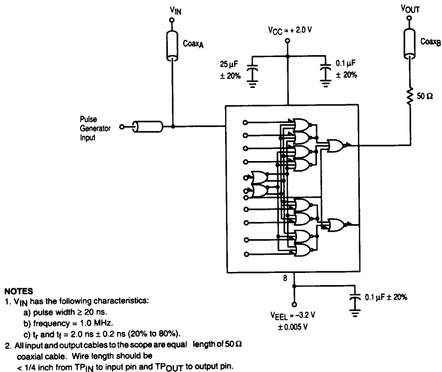
Figure 1. Switching Test Circuit
