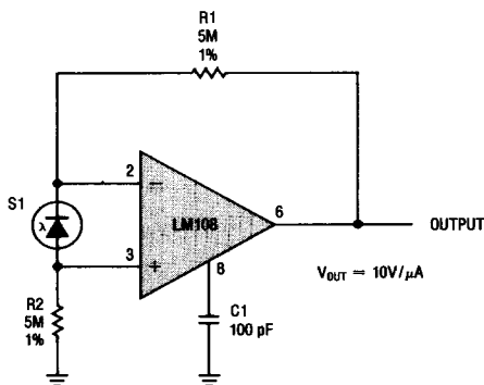
Amplifier For Photodiode Sensor
