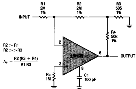
Inverting Amplifier With High Input Resistance
