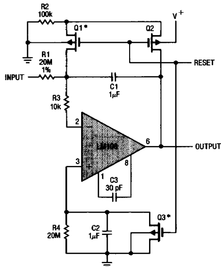
Low Drift Integrator With Reset
