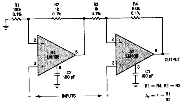
Differential Input Instrumentation Amplifier
