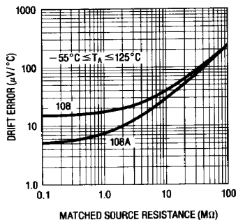
Guaranteed Drift Error
