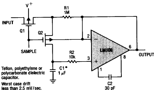
Sample and Hold
