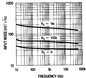
Input Noise Voltage
