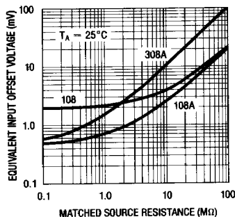
Guaranteed Offset Error
