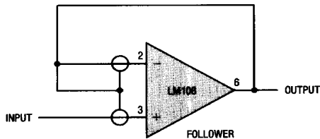
FOLLOWER
