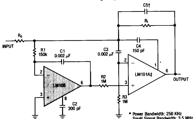
Fast* Summing Amplifier
