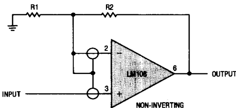
NON-INVERTING
