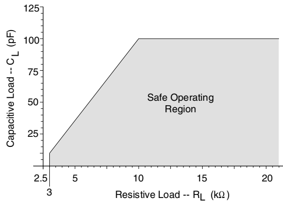
Figure 3. Maximum Loading
