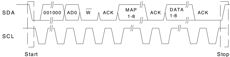
Figure 19. I 2 C Write
