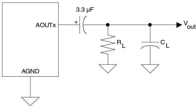
Figure 2. Output Test Load
