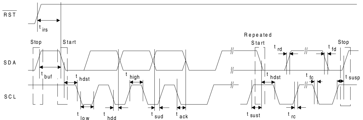
Figure 13. Control Port Timing - I 2 C Mode
