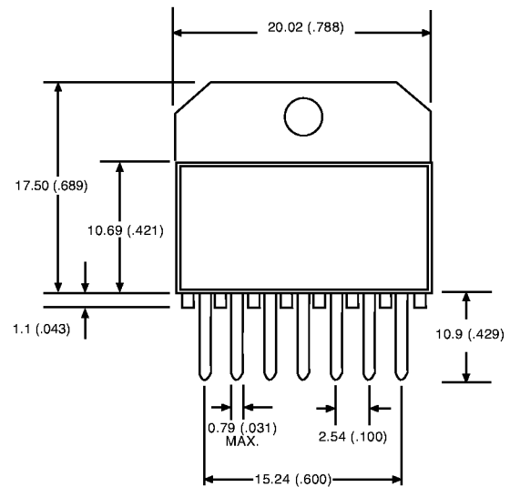
7 Lead Power SIP
