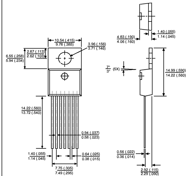
7 Lead TO-220 Straight
