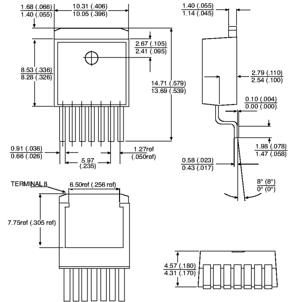
7 Lead D 2 PAK
