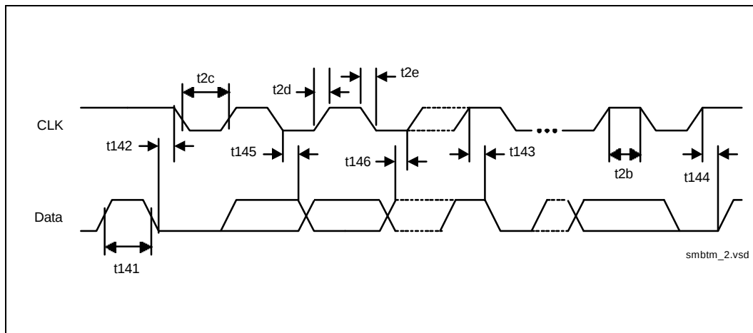
Figure 40. SMBus Timing
