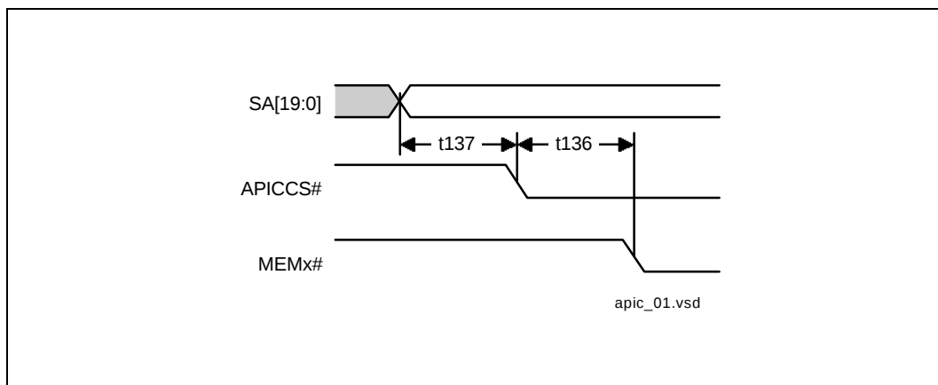
Figure 39. PIIX4 to IOAPIC Timing
