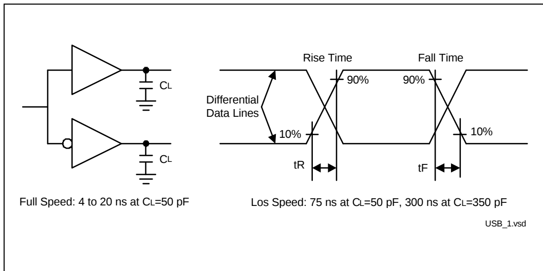
Figure 36. Data Signal Rise and Fall Time
