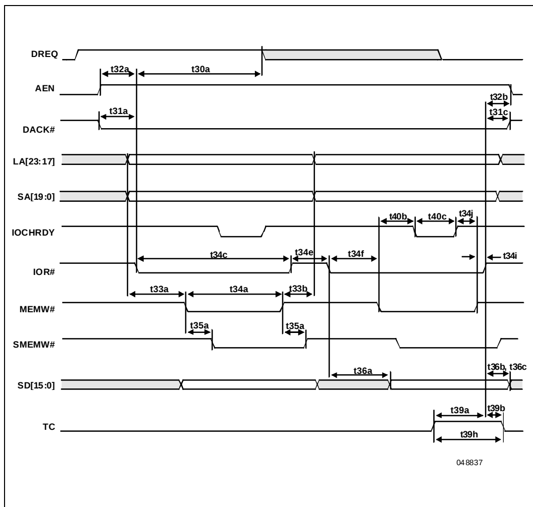
Figure 19. DMA Compatible Timing (Memory Write)
