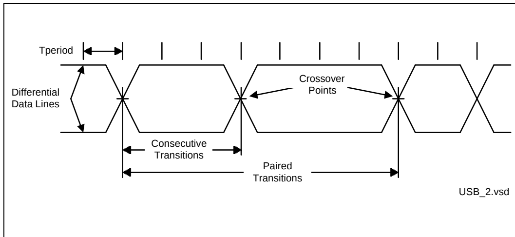
Figure 37. Data Jitter
