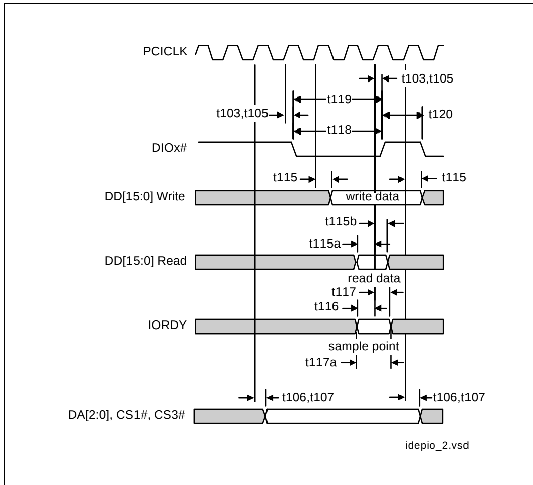
Figure 34. IDE PIO Mode
