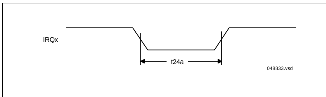
Figure 15. Interrupt Timing
