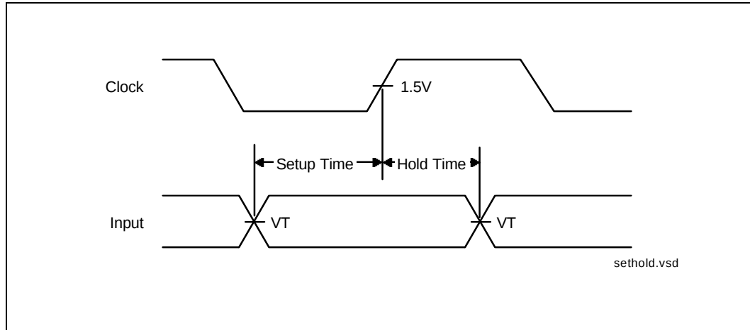
Figure 30. Setup and Hold Times
