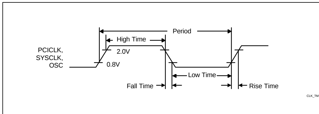
Figure 2. Clock Timing
