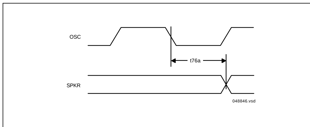
Figure 27. Speaker Timing
