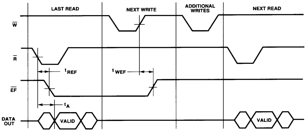
Figure 4. Empty Flag Timing
