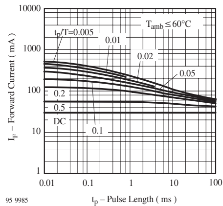
Figure 3. Pulse Forward Current vs. Pulse Duration
