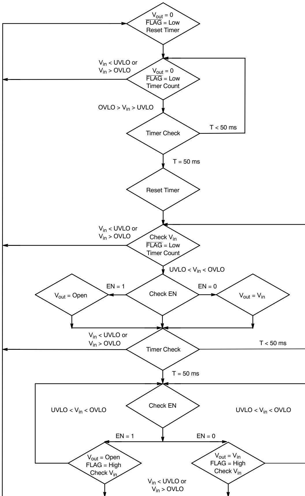
Figure 18. State Machine
