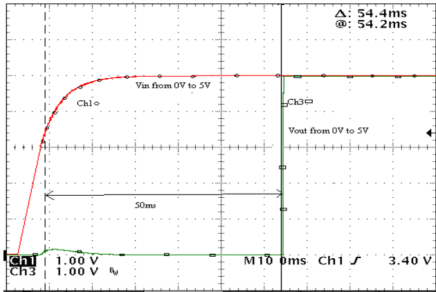
Figure 7. Startup V_{in} = \text{Ch1}, V_{out} = \text{Ch3}
