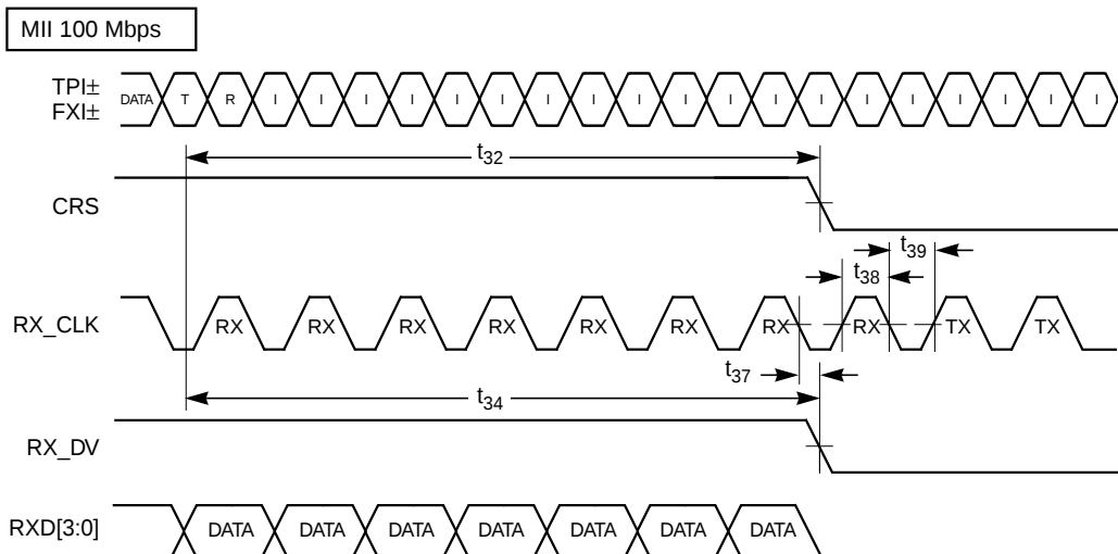
Figure 20 Receive Timing, End of Packet - 100 Mbps
