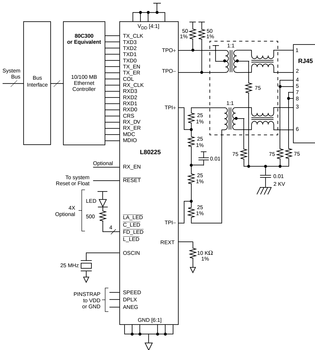
Figure 11 Typical Network Interface Card Schematic Using L80225
