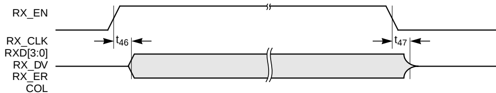
Figure 23 RX_EN Timing
