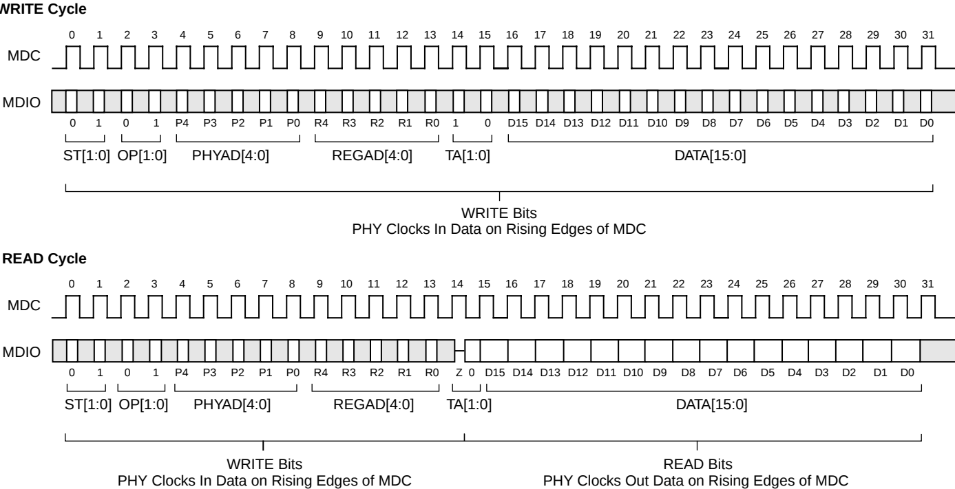
Figure 9 MI Serial Port Frame Timing Diagram
